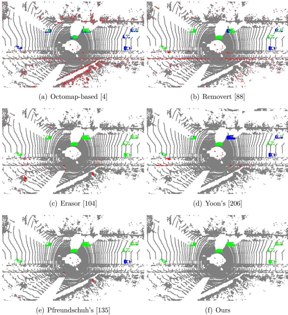
Figure 7.3: Qualitative results of (a) Octomap-based [4], (b) Removert [88], (c) Eraser [104], (d) Yoon's [206], (e) Pfreunds Schuh's [135], and (f) ours. The green points represent the true dynamics (TD), red points are false dynamics (FD), blue points are false statics (FS), and the gray background are true statics (TS).
