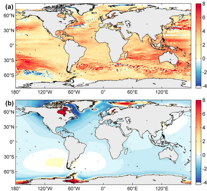
Figure 3. Trend patterns (mm/year) showing changes in water depth: (a) geocentric sea level trends measured by altimetry and (b) Glacial Isostatic Adjustment-induced crustal motions from ICE-6G_C.
