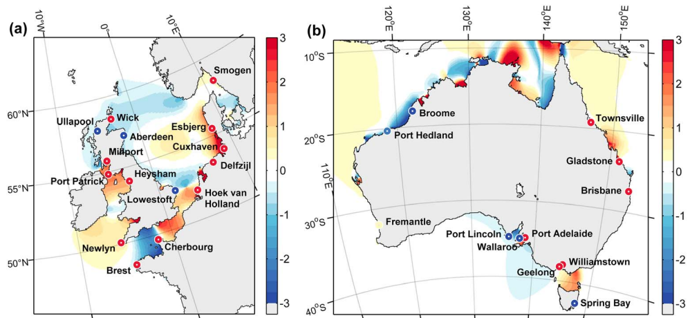
Figure 6. M_2 tidal changes (cm) as in Figure 5 but for (a) the European Shelf and (b) the coastal waters of Australia, hosting another 27 tide gauge stations.
