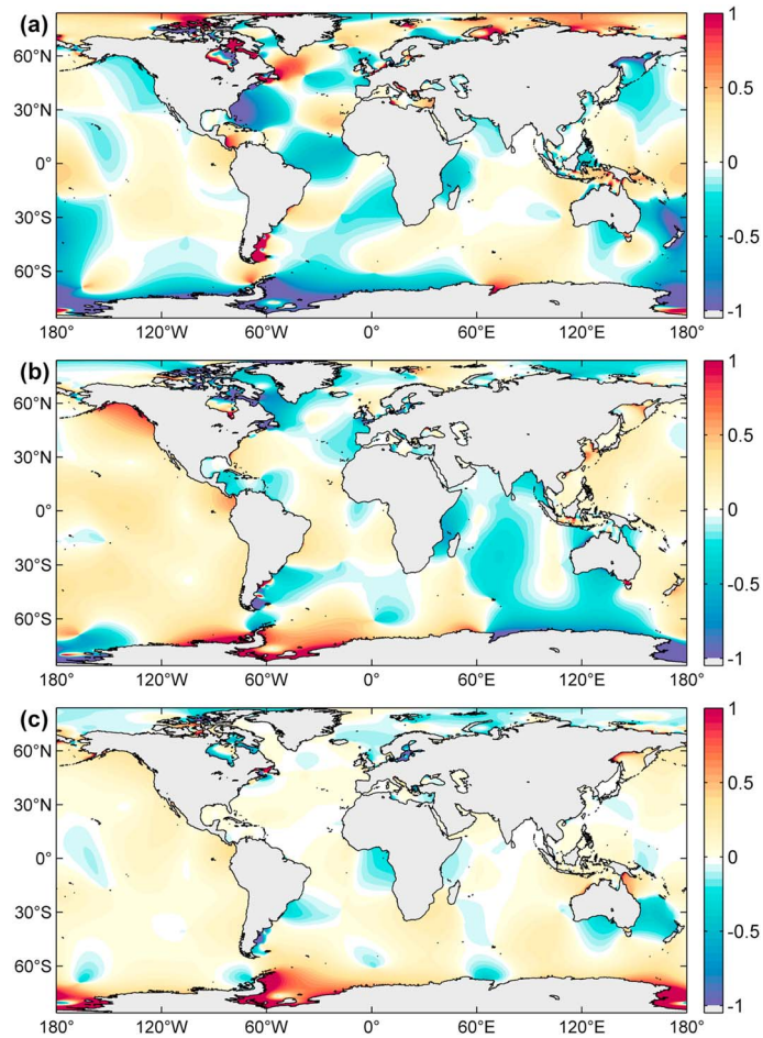
Figure 2. Difference in M_2 amplitudes (cm) between the self-attraction and loading-online control run and an iterating simulation initialized by \beta = 0.10 . Panels show differences after (a) three, (b) four, and (c) five iterations. As in Egbert et al. (2004), the iterative procedure employs a memory term for rapid convergence. Global-mean root mean square errors in deep (shallow) water are 5.1 cm (17.0 cm) for the control run and 5.1 cm (17.1 cm) after five iterations.
