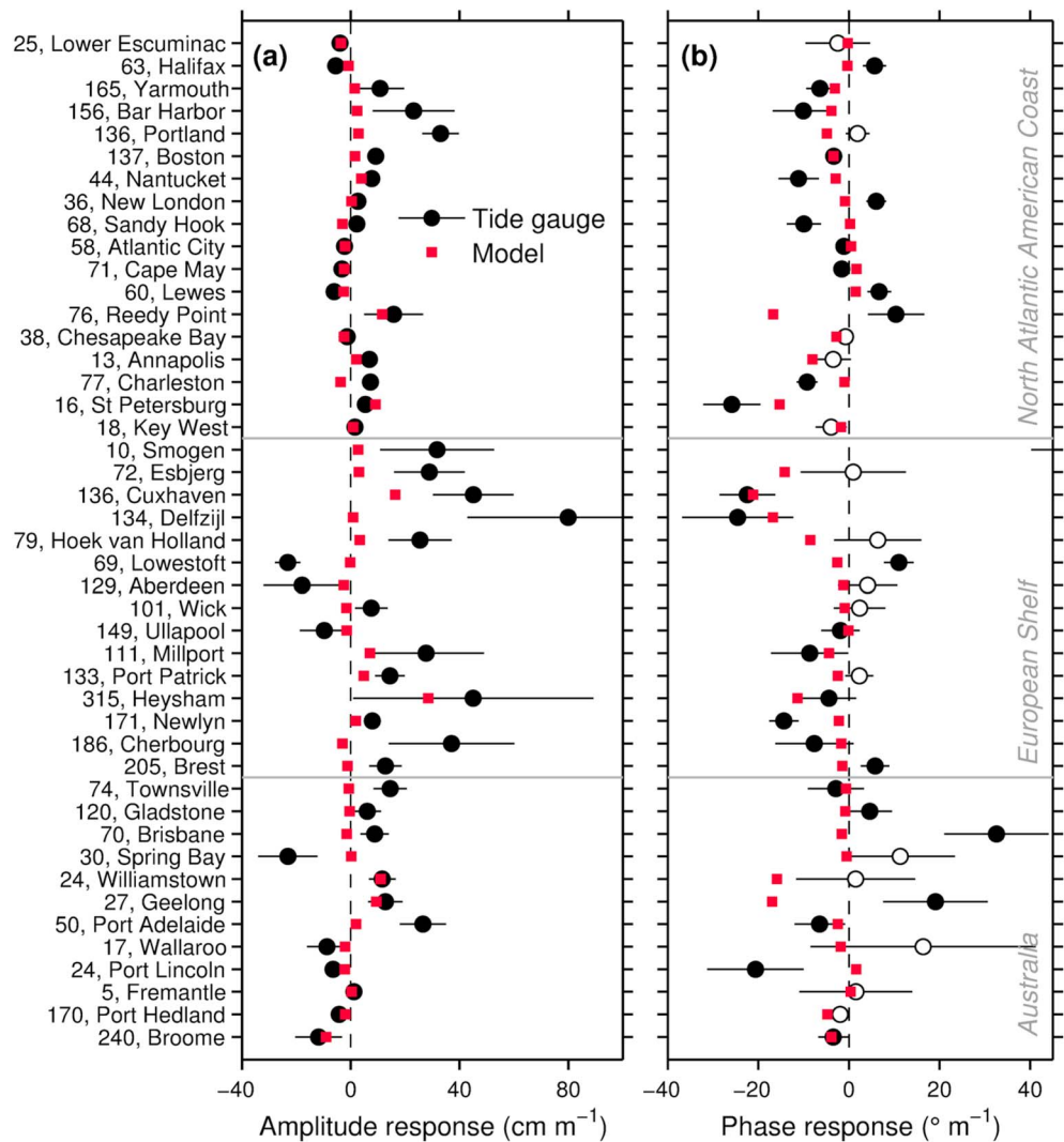
Figure 7. Observed and modeled M_2 response coefficients in (a) amplitude H and (b) phase lag G per meter of sea level rise. Model values are based on simulations using spatially varying depth changes averaging 0.5 m. Error bars correspond to two standard deviations and were propagated from the trend analyses of sea level and annual tidal estimates. Stations with insignificant phase trends (at the 95% confidence level) are shown as white markers in panel (b). Numbers to the left of the station labeling indicate mean M_2 amplitudes.
