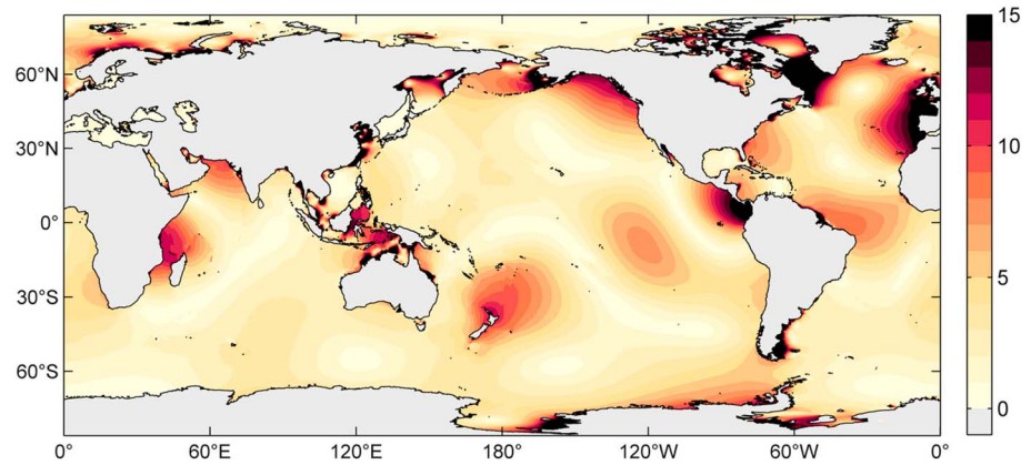
Figure 1. M_2 RMS elevation error (cm) between the TPX08 atlas and our 1/12^\circ simulations based on online evaluation of self-attraction and loading and a scale factor of \kappa_w = 0.3 applied to the conversion scheme. Corresponding global-mean RMS errors are 4.4 cm for depths greater than 1,000 m and 14.6 cm in shallow oceans. RMS = root mean square.
