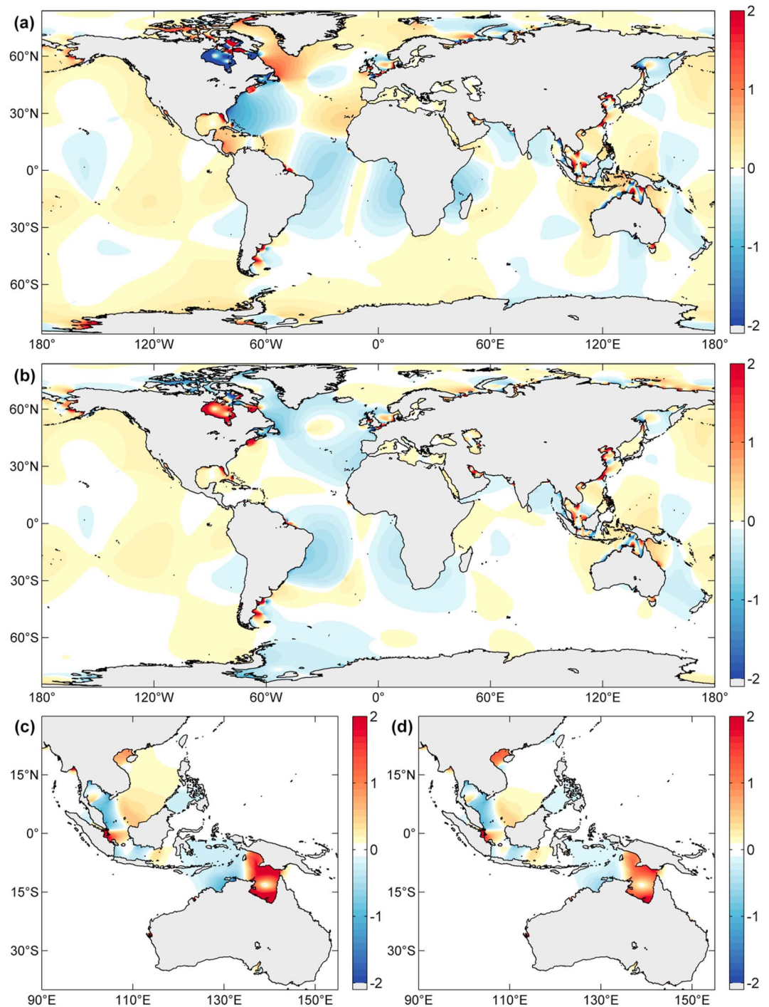
Figure 4. Modeled response of M_2 (a, b) and regional K_1 (c, d) tidal amplitudes (cm) to a 0.5-m increase in global mean sea level based on two different scenarios: (a, c) nonuniform sea level rise with Glacial Isostatic Adjustment and geocentric trends extrapolated from Figure 3 and (b, d) spatially uniform sea level rise.
