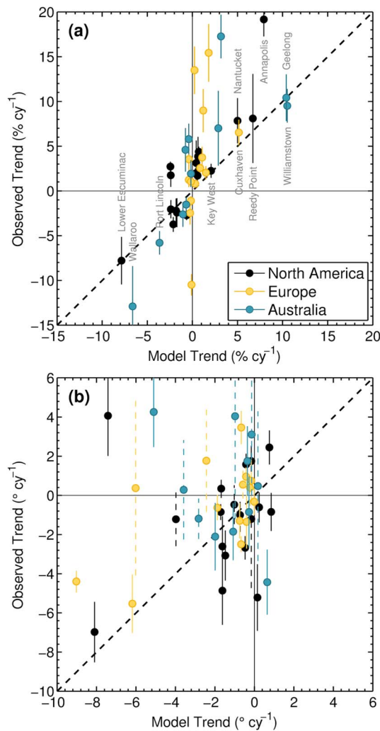
Figure 9. Comparison of observed and modeled M_2 trends in (a) relative amplitude (%/cy) and (b) phase ( ^\circ /cy) at 45 tide gauge stations in North America (black markers), Europe (yellow), and Australia (blue). Stations St. Petersburg, Smogen, and Spring Bay are off the scale in panel (a); see the supporting information for respective tabulations. Error bars of the observed tidal trends correspond to two standard deviations and are shown as dashed lines in panel (b) for stations with insignificant phase trends. Labels in (a) signify locations of particularly large model trends.
