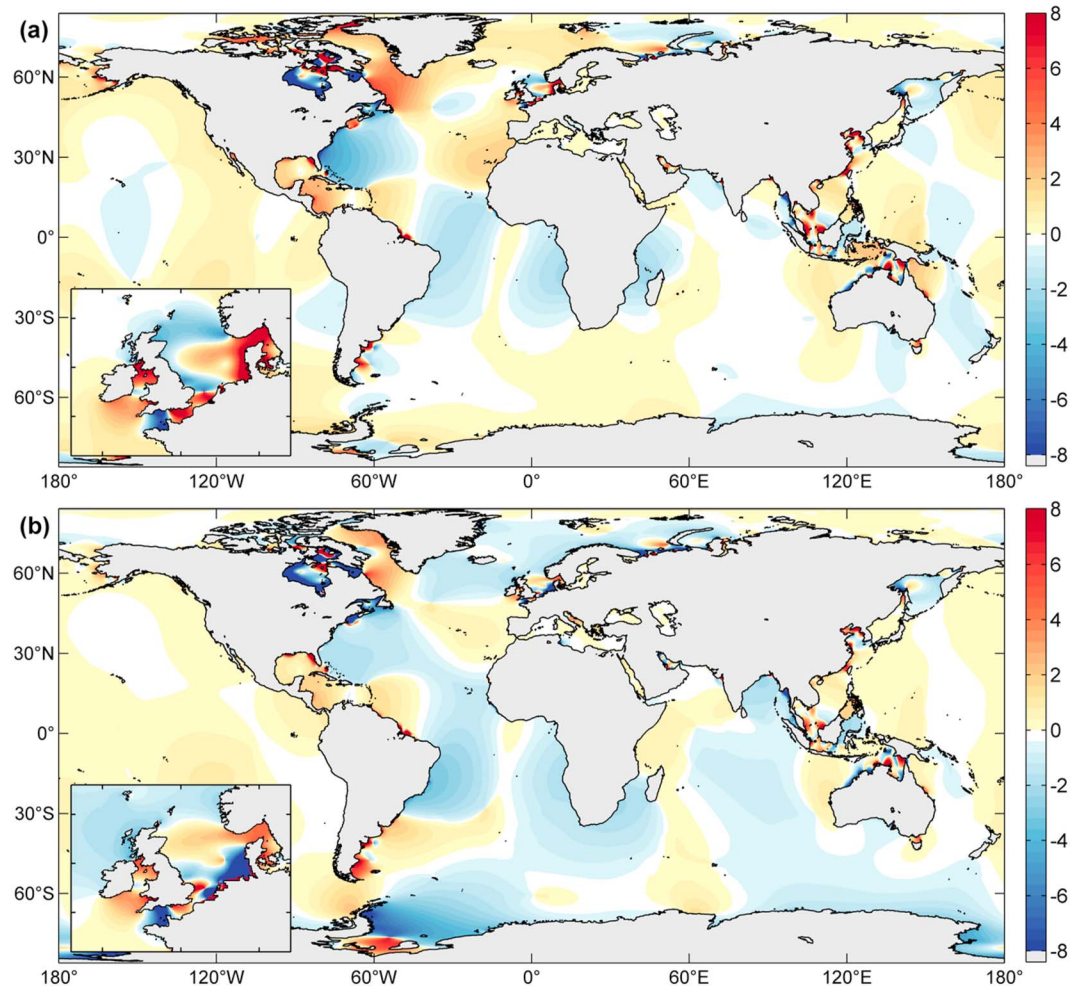
Figure 10. Change in M_2 amplitudes (cm) with an average of nonuniform sea level rise of 2 m, assuming (a) fixed coastlines, and (b) inundation of low-lying land. Respective close-ups of the European Shelf are shown on the bottom left of each panel.
