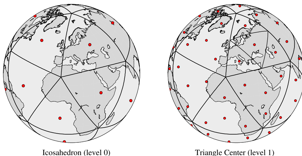
Figure 3.4: Construction of the grid triangle center
