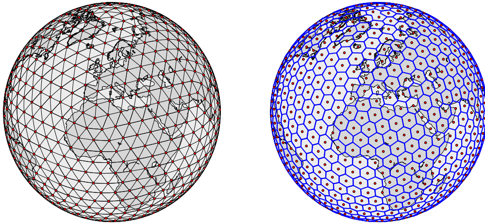
Figure 3.10: Delaunay triangulation (left) and Voronoi diagram (right) of a triangle vertex grid, level 8
