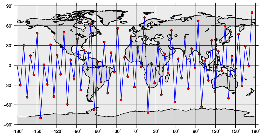
Figure 3.6: Points generated by quasi random grid
