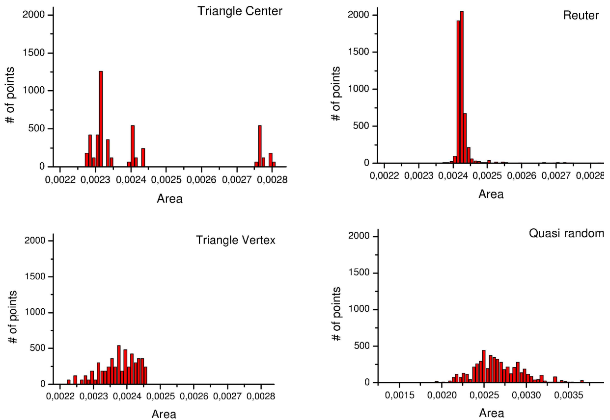
Figure 3.11: Histogram of area sizes associated with individual grid points (different scale for quasi random grid)
