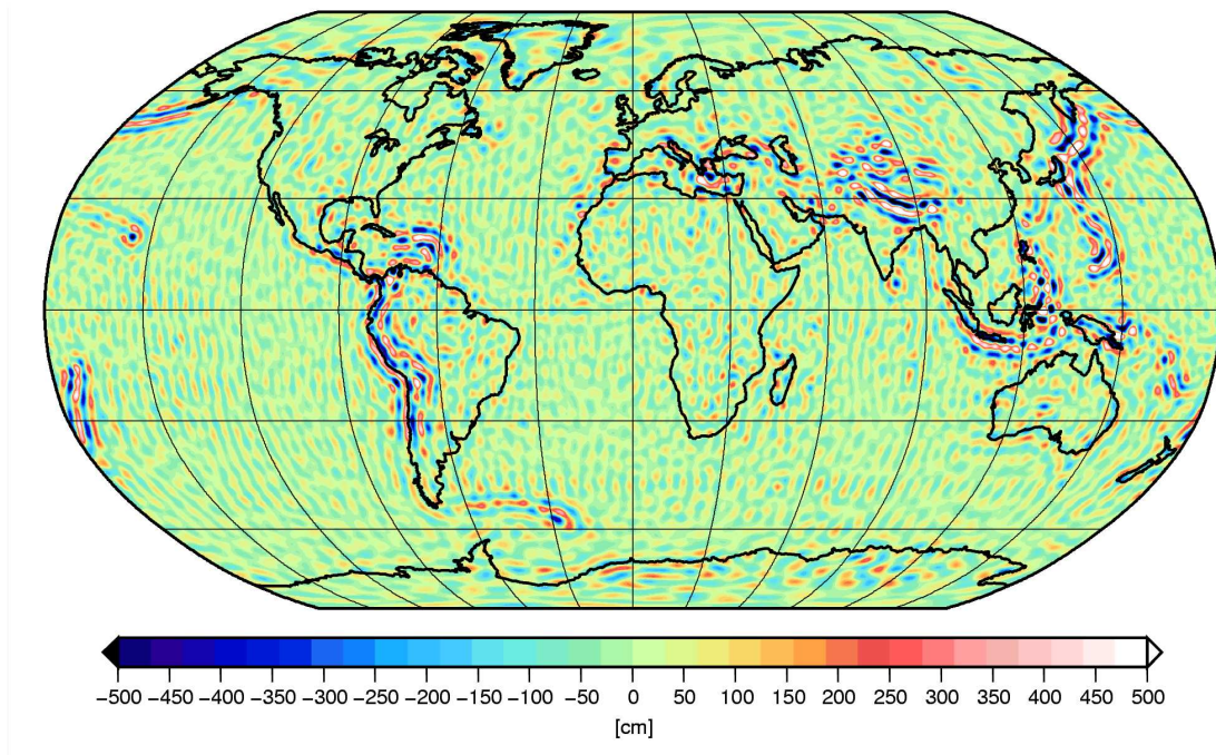
Figure 7.10: Differences between ITG-Champ01k ( N = 70 ) and GGM01s (compared up to degree N = 120 ), RMS: 95.57 cm, Max: 1031.04 cm
