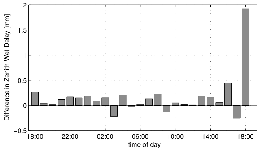
(c) Wetzell: ZWD differences due to constraints in Ny Ålesund.
