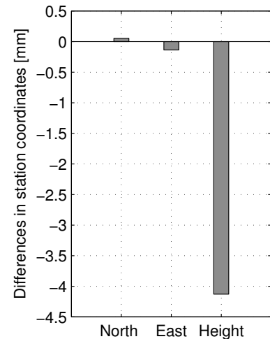
(b) Ny Ålesund: Coordinate differences due to constraints on the ZWDs.
