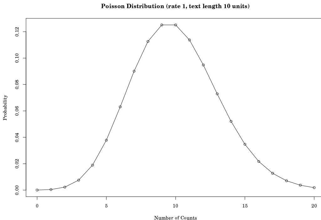
Figure 5.8. Poisson distribution with \rho x = 10
