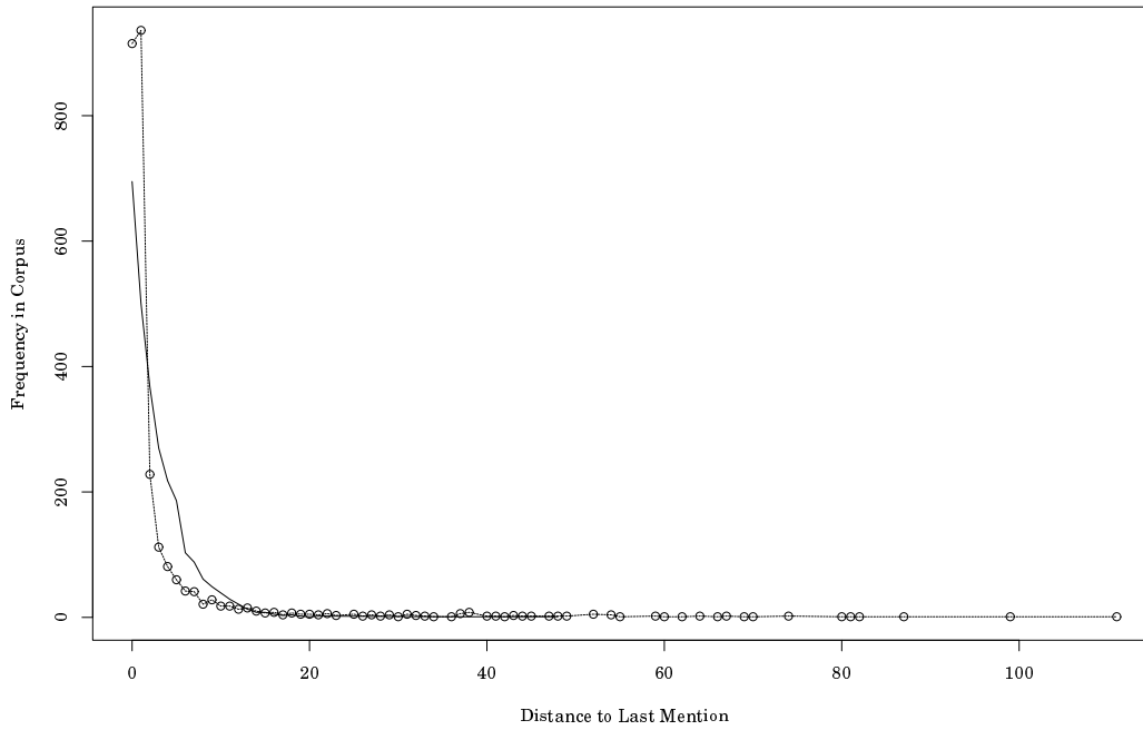
Empirical vs. Predicted Distribution of Distances, Exponential Distribution Model
