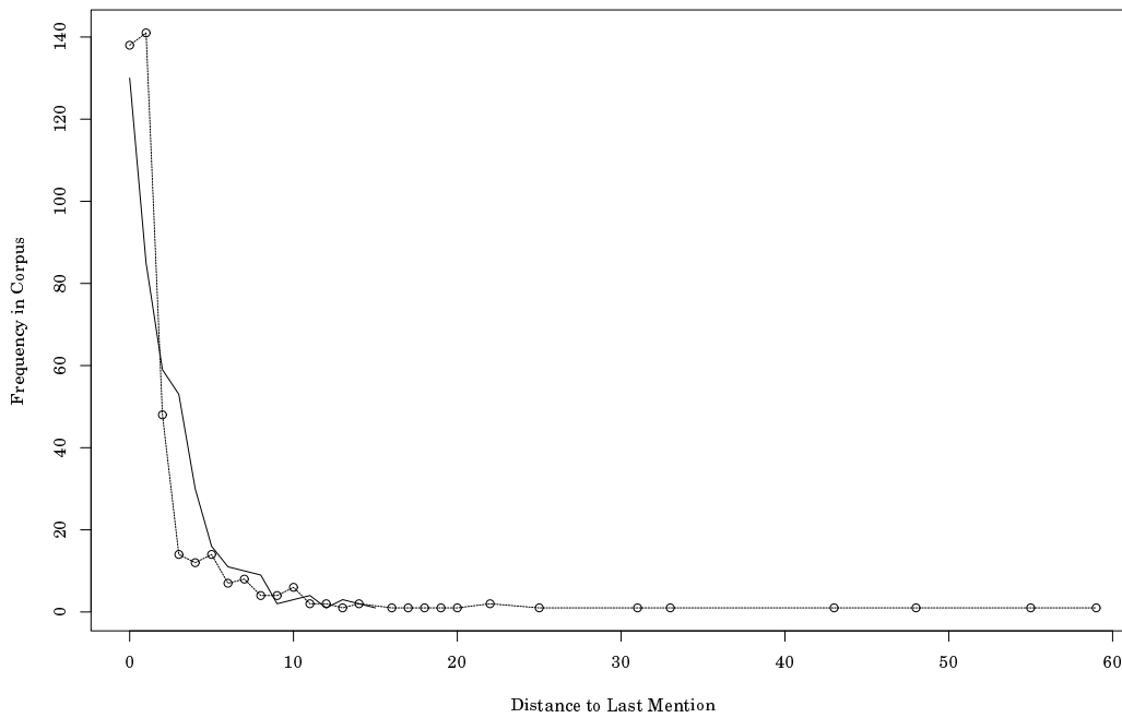
Figure 5.5. Fit of exponential distribution to the data — predicted distances (straight line) versus empirical distances (connected dots). Upper figure: complete corpus, lower figure: Genre CG, best fit
