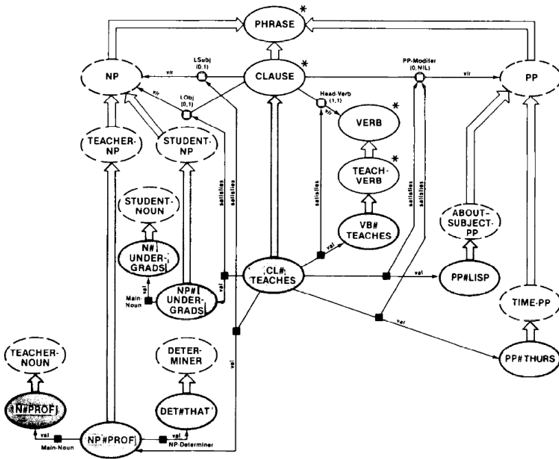
Figure 3.16: A network representing a sentence in KL-ONE (from Brachman and Schmolze, 1985, p. 214).
