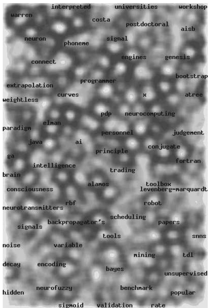
Figure 3.7: WebSOM example: the map of articles from usenet group comp.ai.neural-nets . The labels denote sample posts from the group. Similar articles are placed near each other on the map (topology preserving property). The color represents the density of documents: light areas contain more documents. (From: http://websom.hut.fi/websom/ .)
