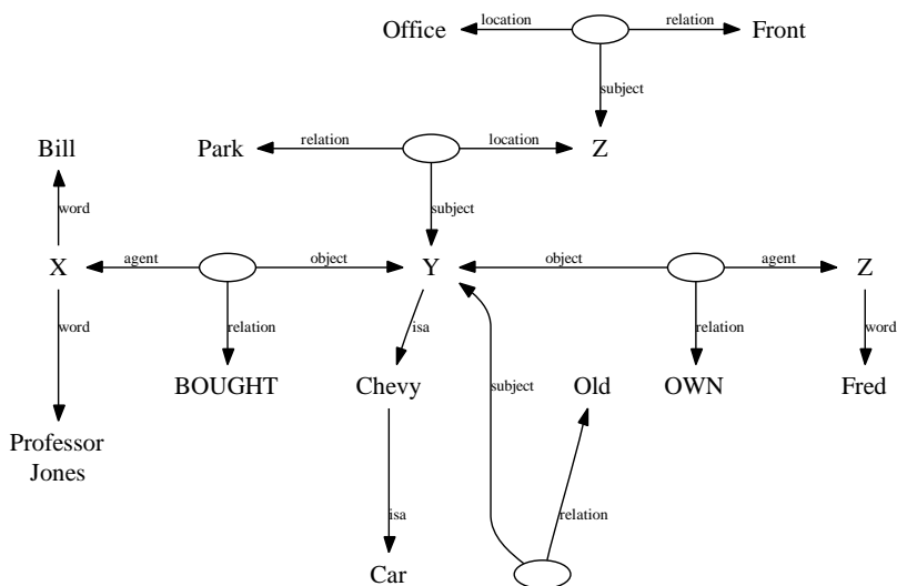
Figure 3.14: A propositional network representing a structure on the sentence level.
