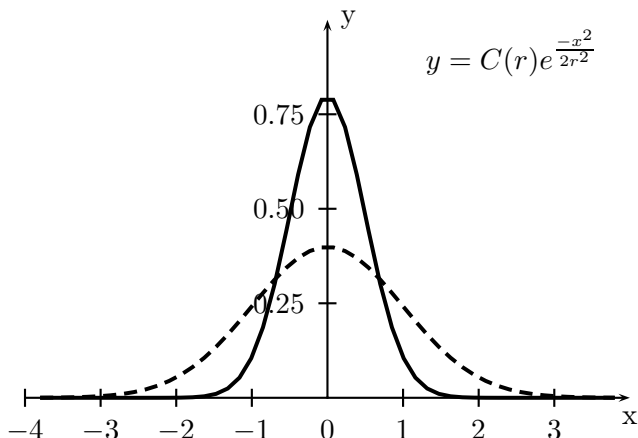
Figure 4.3: Example Gaussian functions: solid line with r = 0.5 , dashed line with r = 1.0
