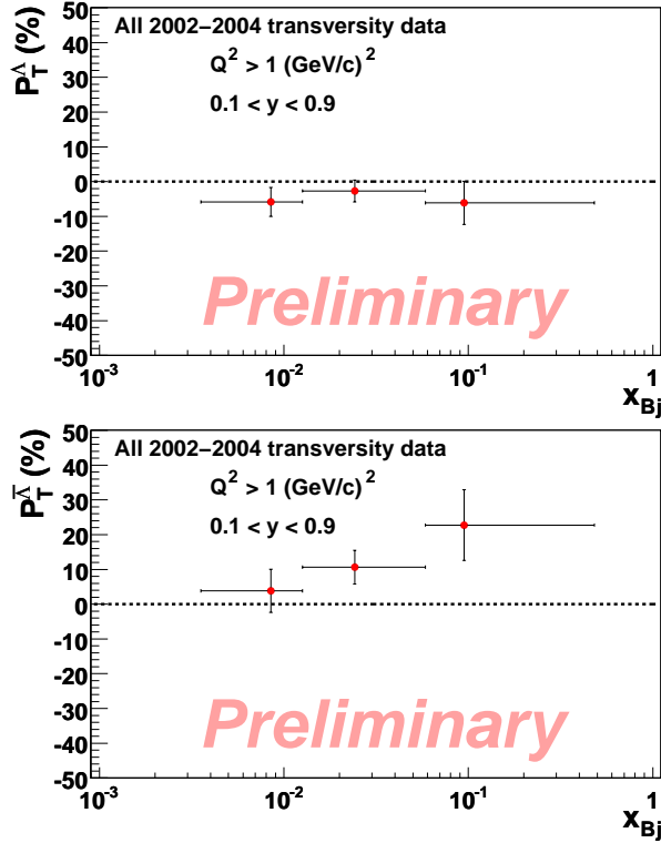
Figure 6.2: \Lambda and \bar{\Lambda} polarizations with statistical errors as a function of x_{Bj} in the 2002-2004 COMPASS data on a transversely polarized deuteron target with Q^2 > 1 (GeV/c) ^2 and 0.1 < y < 0.9 [121].
