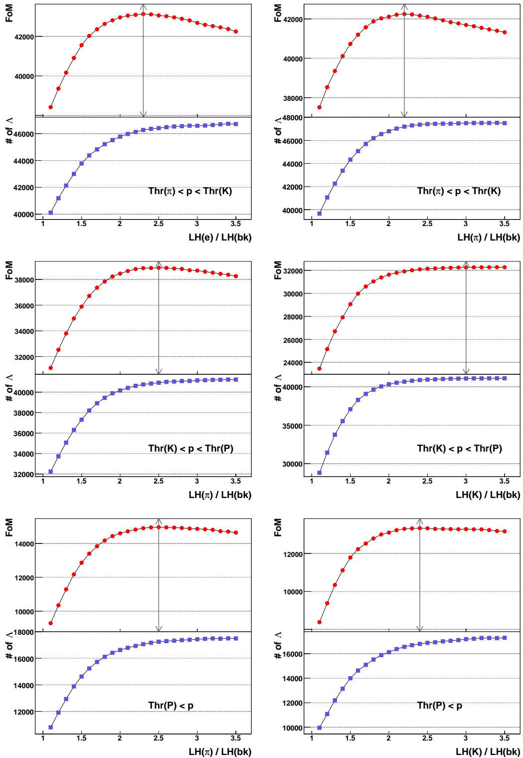
Figure 4.8: Figure of Merits (FoM) in the range of momentum at \text{Thr}(\pi) < p < \text{Thr}(K) , \text{Thr}(K) < p < \text{Thr}(p) , and \text{Thr}(p) < p for \Lambda selection.
