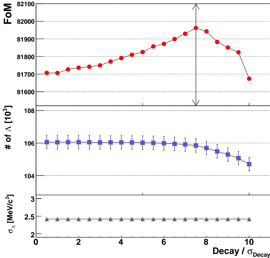
Figure 4.3: The Figure of Merit ( FoM = \frac{S^2}{S+B} ), number of \Lambda particles, and the mass resolution \sigma_{\Lambda} from the Gaussian fit of the invariant mass distributions with application of the D > x \cdot \sigma_D cut in a range from x = 0 to 10 are shown. The grey arrow in the top panel indicates the optimized value of the FoM at D > 7.5\sigma_D .
