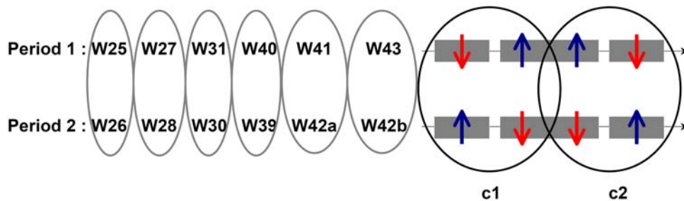
Figure 5.7: Definition of the split six target-periods configuration used to estimate systematic effects. The red arrows display the target spin orientation downwards, while the blue arrows state the target spin orientation to be upwards [66].
