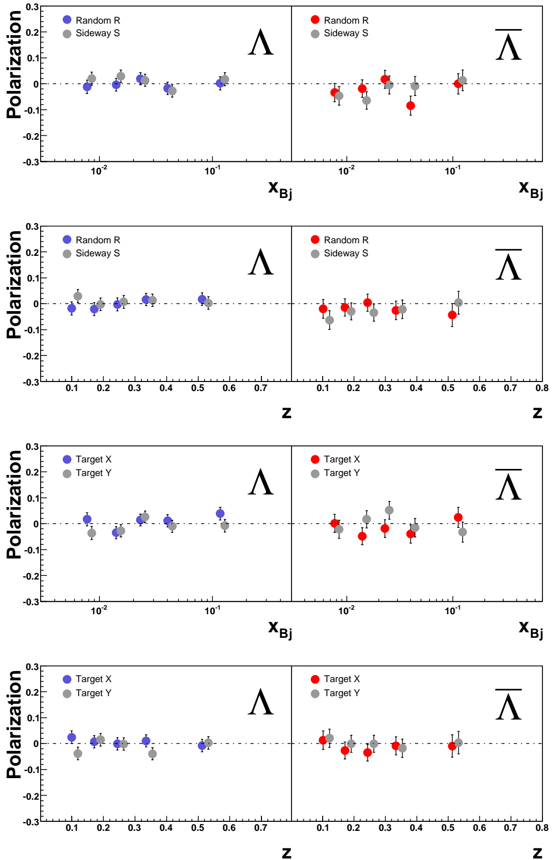
Figure 5.11: In the top two panels, the results of polarization with random and sideway target spin orientation are given. The bottom two panels show the results of polarization with dividing the target in x- and y-direction.
