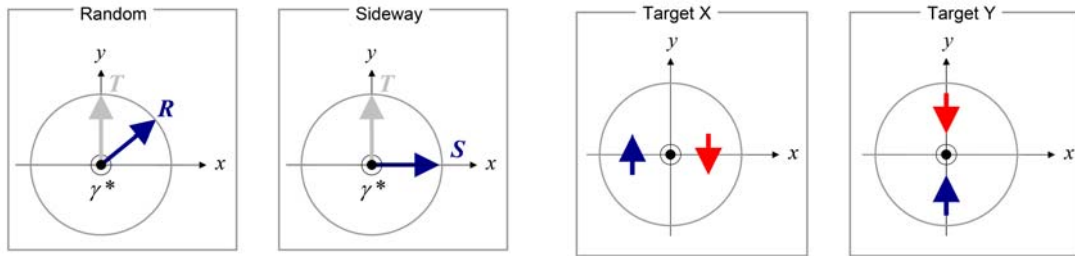
Figure 5.10: From left to right: Definitions of target spin orientation are shown by an event-by-event random rotation Random and a sideway direction Sideway of the target spin in the laboratory system, as well as defined in a geometrical way in the x-direction Target X and y-direction Target Y [66].
