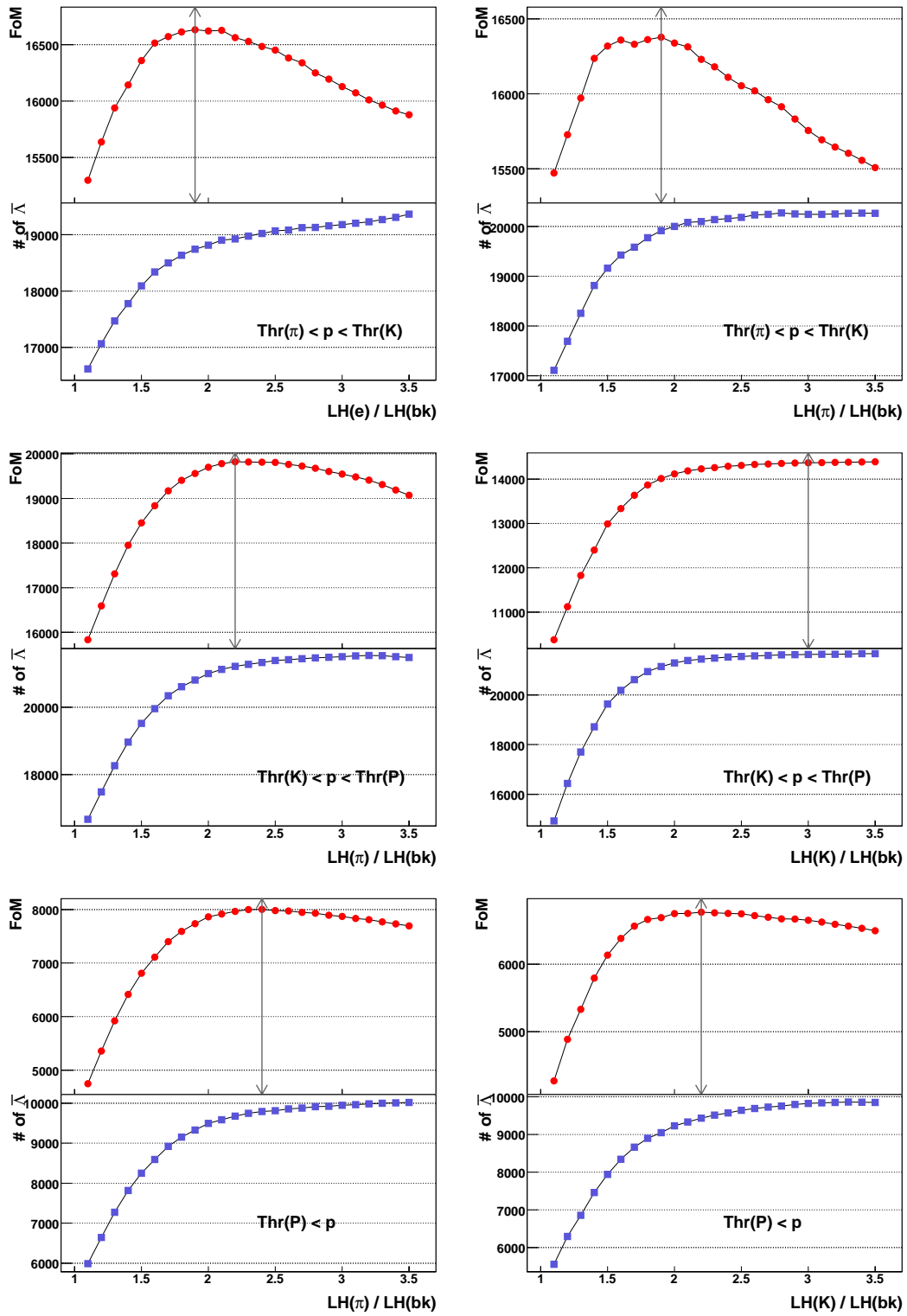
Figure 4.9: Figure of Merits (FoM) in the range of momentum at \text{Thr}(\pi) < p < \text{Thr}(K) , \text{Thr}(K) < p < \text{Thr}(p) , and \text{Thr}(p) < p for \bar{\Lambda} selection.
