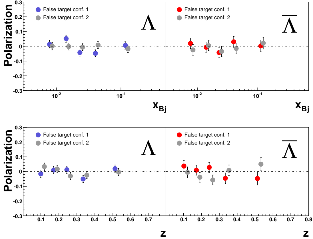
Figure 5.13: Results of polarization with false target configurations.
