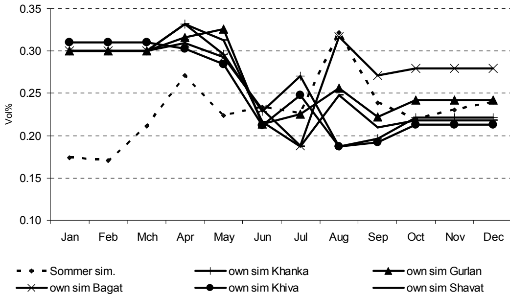
Figure D-2 Plausibility control, comparison of soil moisture, for heavy/loamy soils under cotton cultivation
