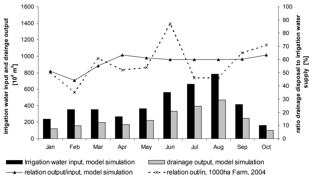
Figure 5-5 Total irrigation water input and drainage output (in 10^6 \text{ m}^3 ) and ratio between drainage disposal and water supply (in %)
