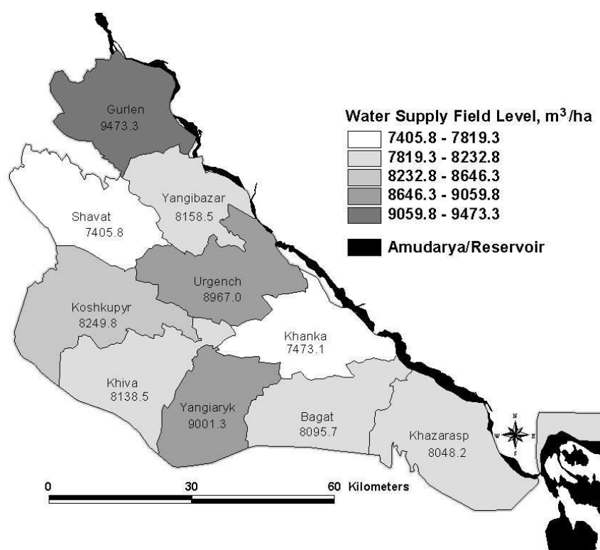
Figure 5-9 Water supply at field level, Khorezm, 2003 (in m 3 /ha)
