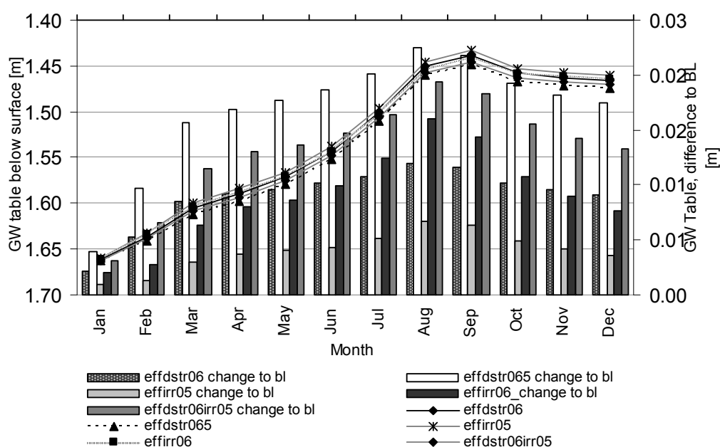
Figure E-1 Groundwater table depth and change compared to Baseline1 for different efficiency experiments under status quo scenario, absolute values (in m)
