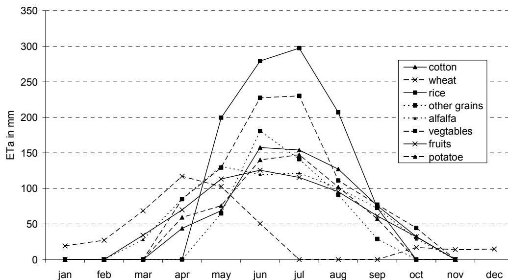
Figure 5-1 Calculated monthly Eta for the Gurlan district with medium soils (sandy-loamy) for different crop types (in mm)
