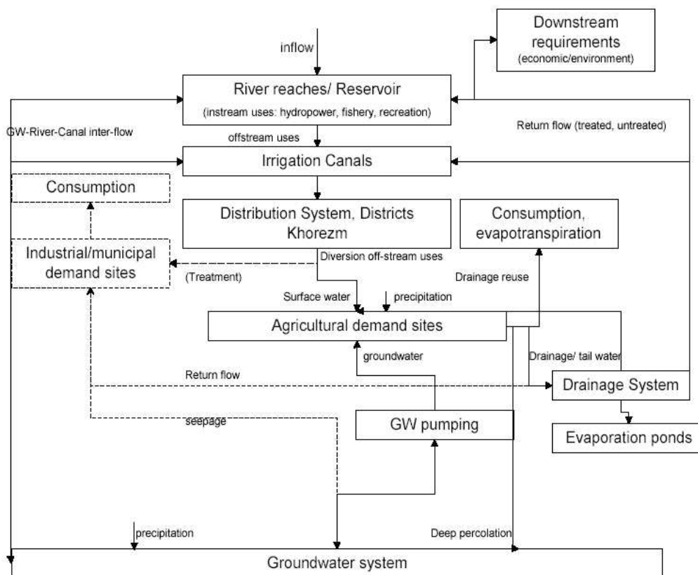
Figure 3-2 Schematic representation of the water distribution process in the Khorezm Water Management Model
