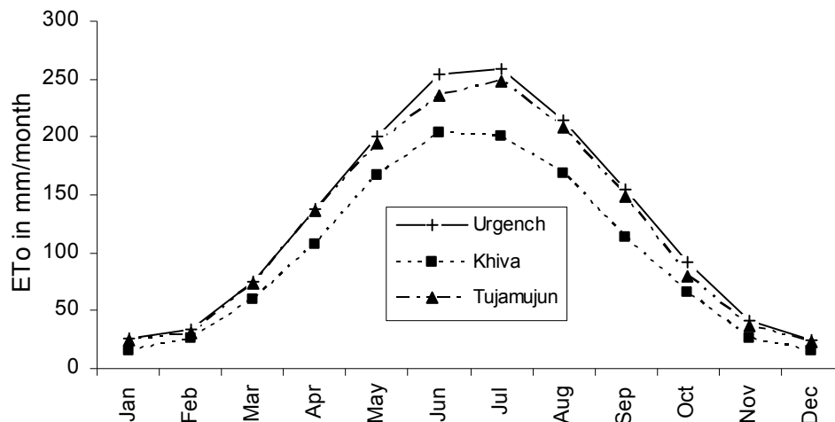
Figure 4-6 Reference evapotranspiration at the main climate stations in Khorezm (mm/month)
