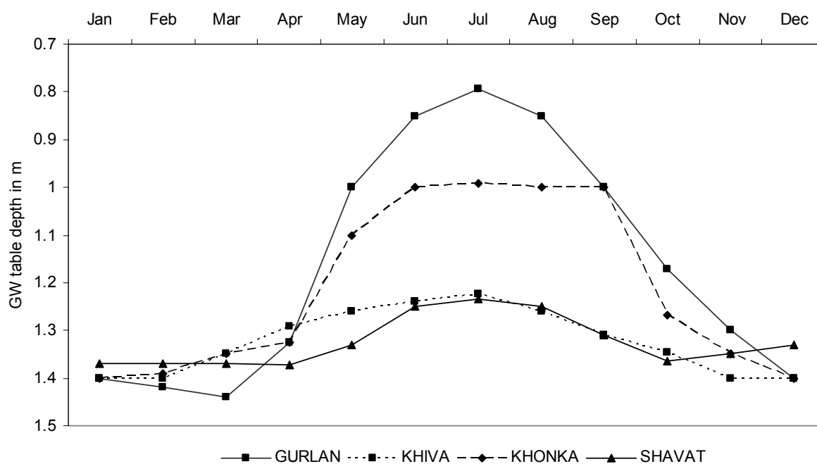
Figure 4-5 Groundwater table in Khorezm for selected districts in 2003 (m)
