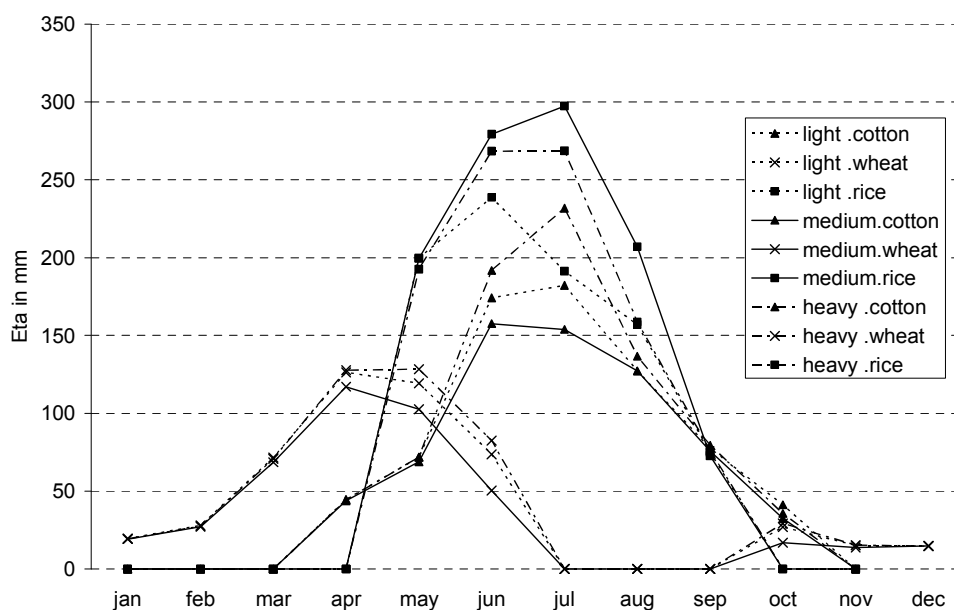
Figure 5-2 Calculated monthly ETa in the Gurlan district, for cotton, wheat and rice, for different soil types (in mm)
