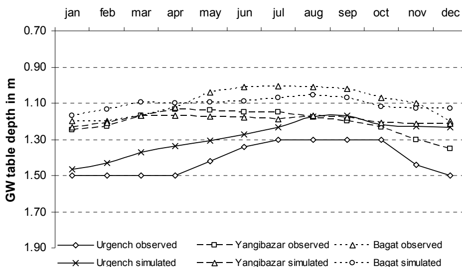
Figure 5-3 Groundwater simulation and verification
