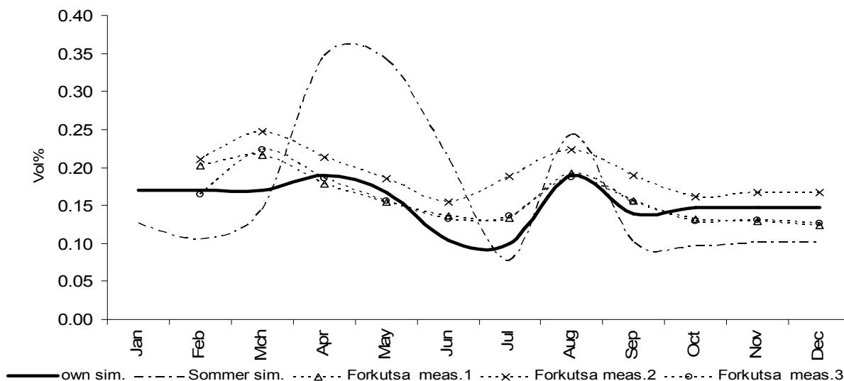
Figure 5-6 Soil moisture for soils under cotton cultivation: plausibility control, exemplified for the Khiva district
