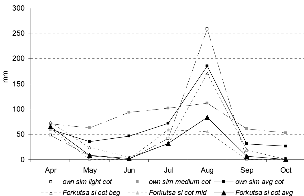
Figure 5-7 Downward water flux (deep percolation) in the Khiva district, plausibility control (in mm)
