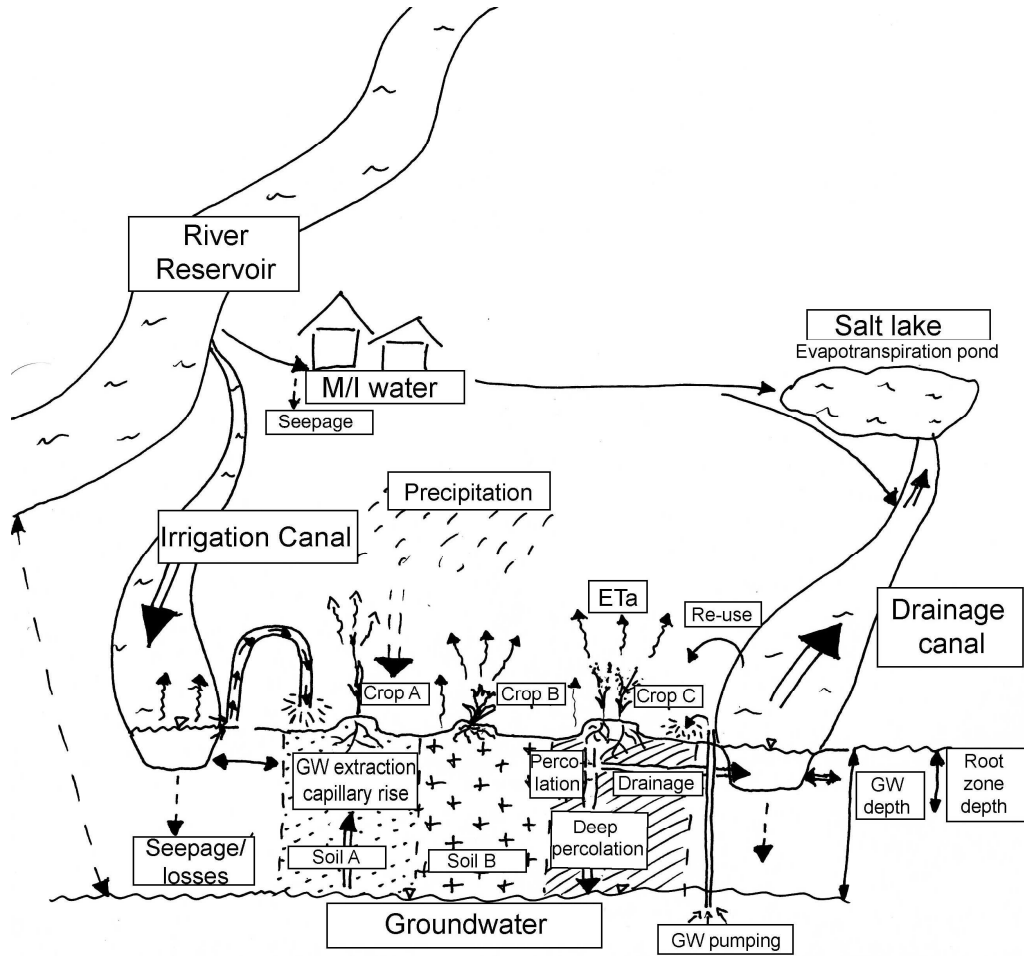
Figure 3-4 Schematic showing the surface and sub-surface water flows and soil water balance used in the model
