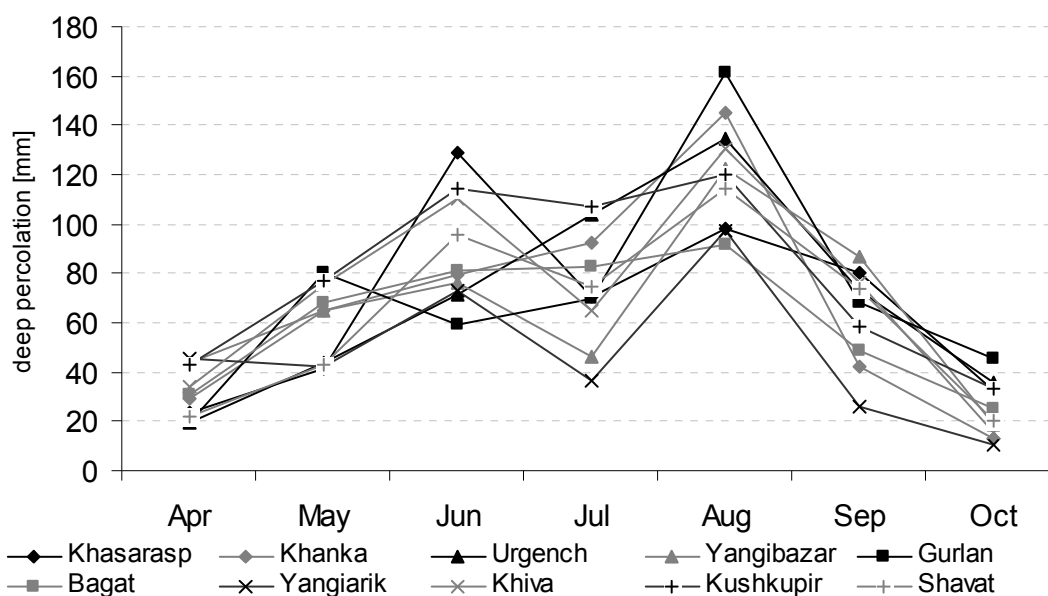
Figure 5-8 Deep percolation per Khorezm district (in mm)
