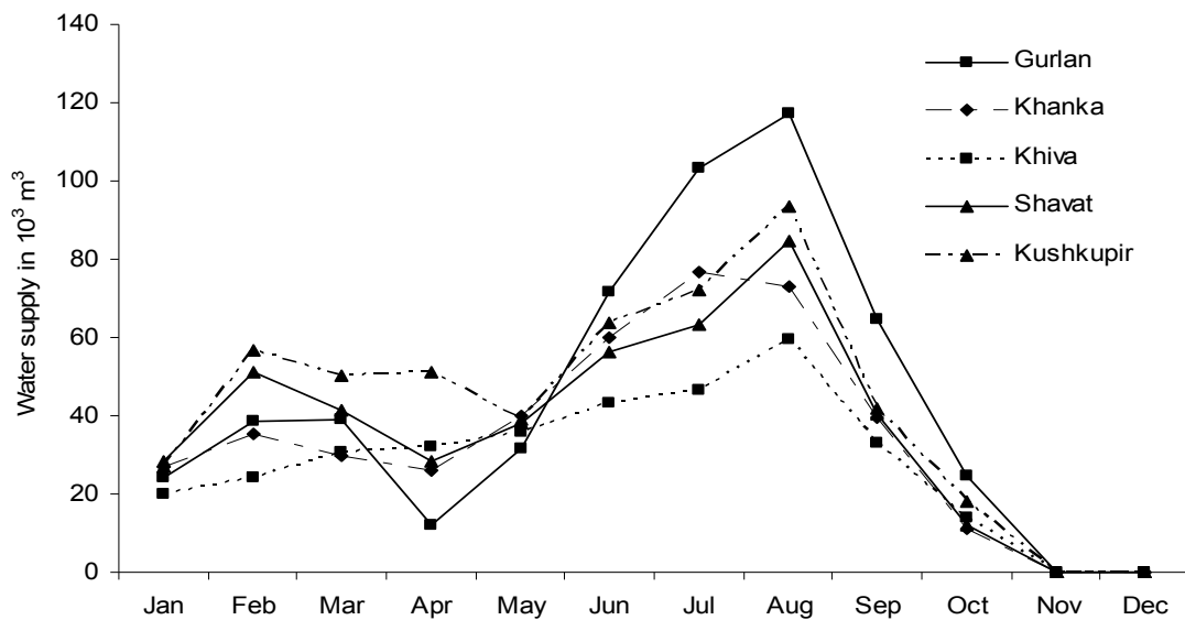
Figure 4-2 Total monthly water supply for selected Khorezm districts in 2003 (10³ m³)
