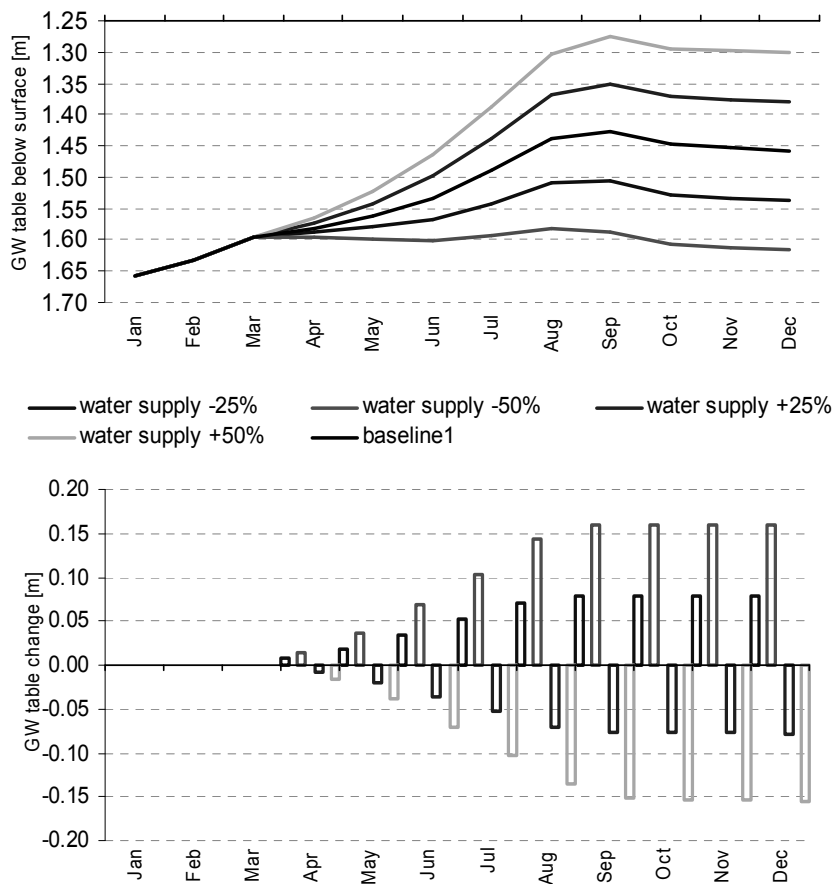
Figure 8-5 Groundwater table depth and GW table difference to Baseline 1 for different water supply experiments averaged over all districts (in m)
