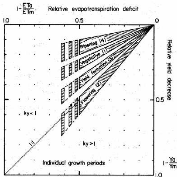
Figure 3-9 Relationship between relative yield and relative evapotranspiration for individual growth periods
