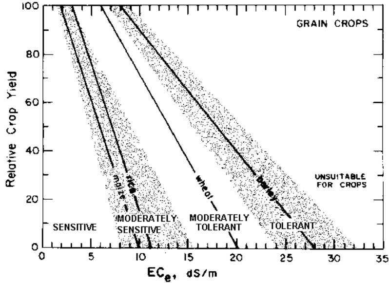
Figure 3-7 Salt tolerance of grain crops
