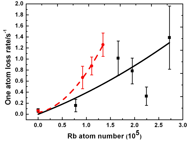
Figure 5.6: The Cs one-atom loss rate is plotted for N_{\text{Cs}} = 1 in the presence of Rb in the |1,0\rangle state (black squares) and |2,0\rangle state (red dots) with their respective fits (black straight lines and red dashes lines). The stronger curvature of the fit for Rb in the |2,0\rangle state indicates a higher quadratic dependence of the loss rate on the Rb atom number. The quadratic dependence is due to the loss rate L_{\text{Cs-Rb-Rb}} as already mentioned before and this is an indication of a higher L_{\text{Cs-Rb-Rb}} value in the presence of Rb in the |2,0\rangle state.
