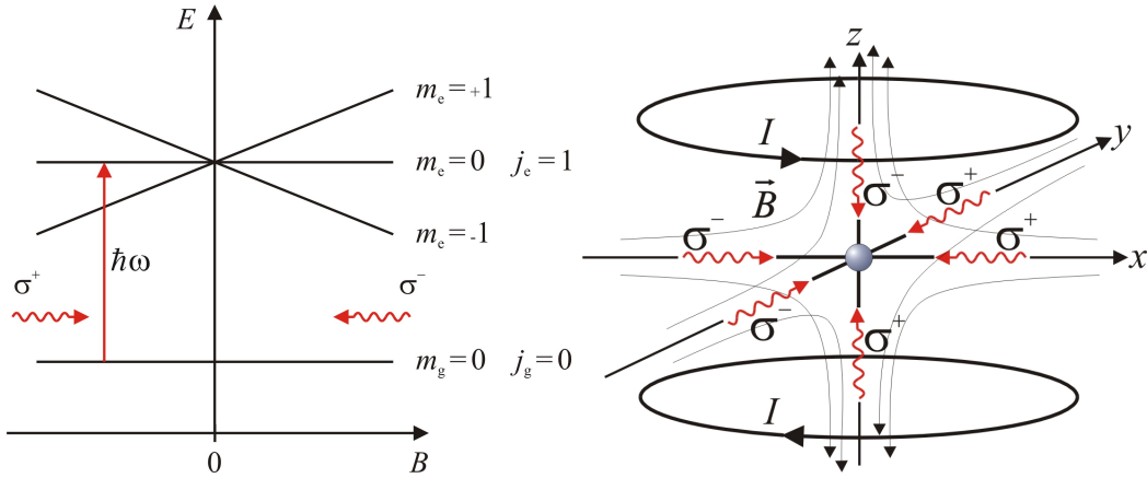
Figure 3.2: The figure on the left shows a 1D picture of the MOT. The upper hyperfine level has three Zeeman states. The two circular polarized light beams \sigma^+ and \sigma^- trap the atoms at B = 0 (see text). An extension in 3D is shown on the right with circular polarized beams in all the six directions.
