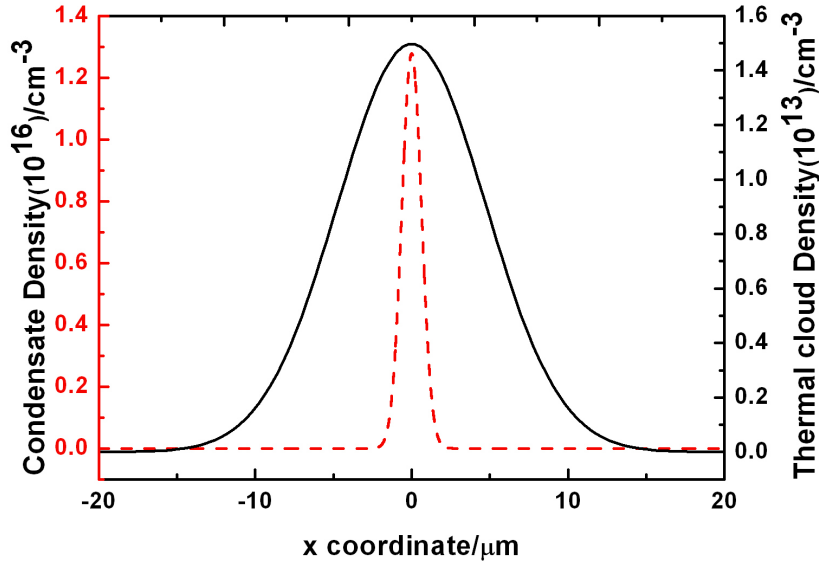
Figure 1.5: The graph shows a cut through the density profile of an ideal Bose condensate (red dashed curve) and a thermal cloud (black curve). As can be seen clearly from the graph, the width of the condensate is much smaller than that of the thermal cloud. Both the curves represent a Gaussian distribution. The curves have been calculated for the trap parameters of our dipole trap (see section 3.7) for a temperature of 200 nK and 10^5 atoms. The peak density of the condensate is three orders of magnitude larger than that of the thermal cloud (as is indicated by the two different scales).
