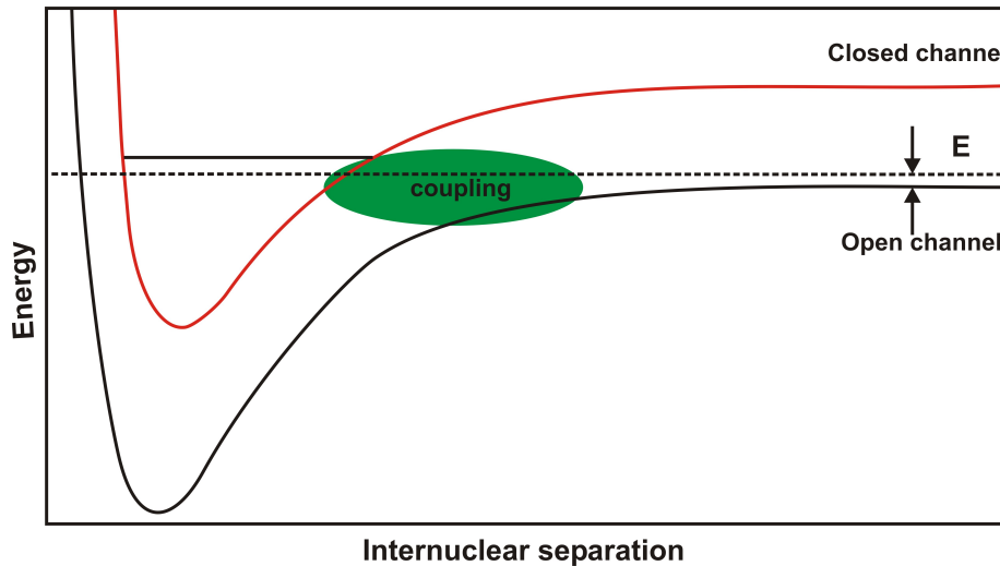
Figure 6.1: A schematic of the molecular potentials of the open (black curve) and closed channel (red curve) are shown. The energy is plotted against the internuclear separation. The atoms collide in the open channel with an energy E . A coupling exists between the two channels. When the energy of the colliding atoms becomes degenerate with the energy of the bound state (shown by the black line) of the closed channel, a quasimolecule is formed in the bound state. This corresponds to a Feshbach resonance.
