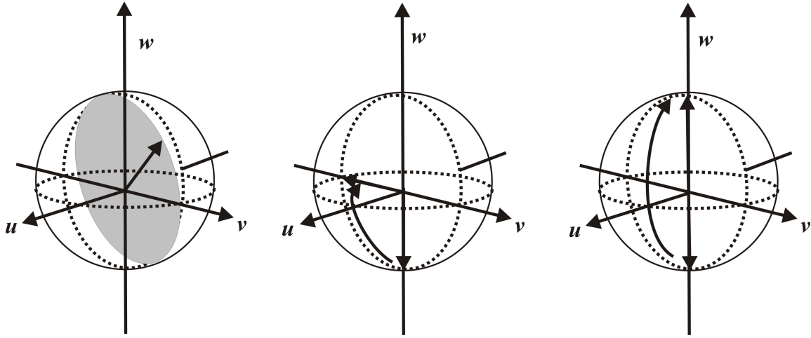
Figure 2.1: The rotation of the Bloch vector \rho on the Bloch sphere is shown. Here, u , v and w correspond to the components of the Bloch vector. The leftmost figure shows the rotation of the Bloch vector about u for a given angle \theta_B at resonance. The middle figure shows the flipping of the Bloch vector onto the horizontal plane for a \pi/2 pulse and the rightmost shows the complete flipping from -w to +w for a \pi pulse.
