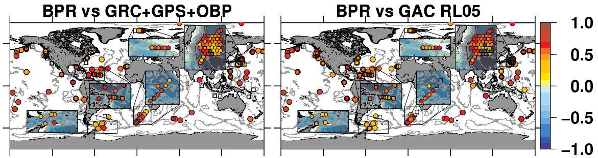
Figure 5.8: Correlation of the inversion solution with in situ bottom pressure series. Circles and triangles denote positive and negative correlations respectively. Empty squares indicate insignificant correlations (based on p-values larger than 0.05, which commonly arise because of a limited time span). Both the combination solution and the GAC product are evaluated up to degree and order 30.
