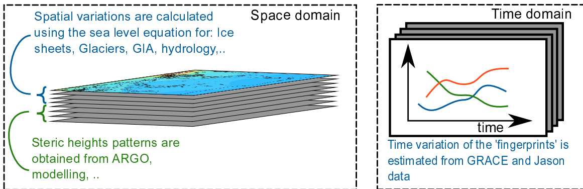
Figure 4.9: Principle of the fingerprint inversion. In the inversion, the spatial patterns are used as base functions. The associated time varying scales are fitted to the data.
