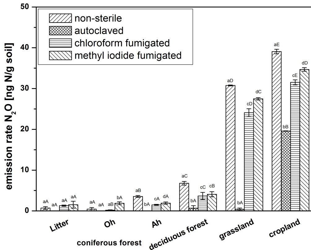
Figure 4.2: N 2 O emission rates in ng N per g soil from six different non-sterile and sterilized soil samples after the addition of NH 2 OH solution (5 nmol) in 6-h incubation experiments. Replicates with the addition of deionized H 2 O were used as backgrounds and subtracted from the results. Error bars represent the SD of three replicates. Lower case letters indicate significant differences between different treatments at one site, capital letters between different sites within one treatment ( \alpha < 0.05 ).
