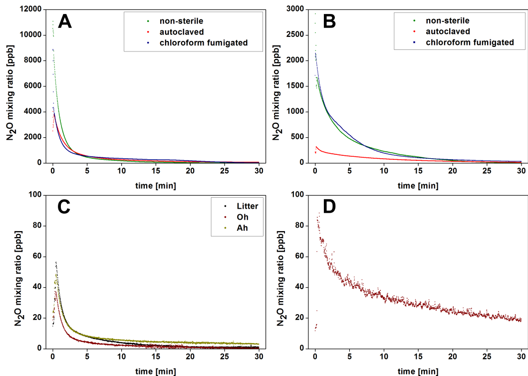
Figure 4.4: N_2O mixing ratios in ppb measured at a temporal resolution of 1 Hz emitted from different soils after the addition of NH_2OH solution ( 5 \mu mol ): (A) from non-sterile and sterile cropland soil, (B) from non-sterile and sterile grassland soil, (C) from the three non-sterile coniferous forest soil layers, and (D) non-sterile deciduous forest soil.
