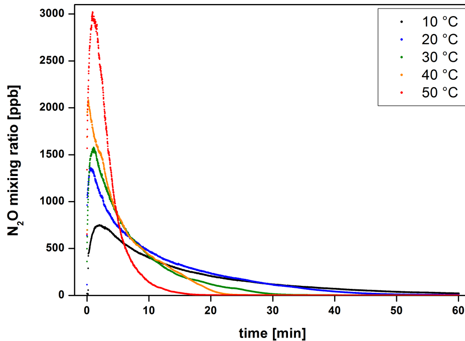
Figure 4.5: N_2O mixing ratios in ppb measured at a temporal resolution of 1 Hz emitted from sterile (autoclaved) cropland soil after the addition of NH_2OH solution ( 5 \mu mol ) at different temperatures from 10 to 50 °C.
