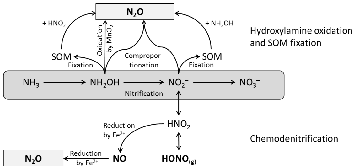
Figure 2.1: Schematic of chemical reactions of nitrification intermediates leading to N 2 O formation (SOM = soil organic matter).
