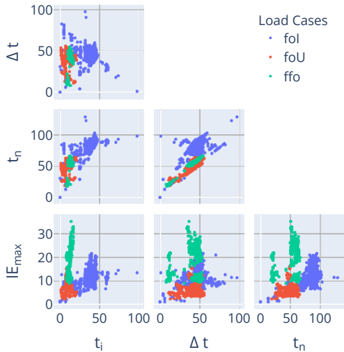
Figure 10: DOE fingerprint load-case scheme, five most energetic components in simulations from four development stages. Simulation specification in Table 1 ( t_i [ms], \Delta t [ms], IE_{max} [kNmm])
