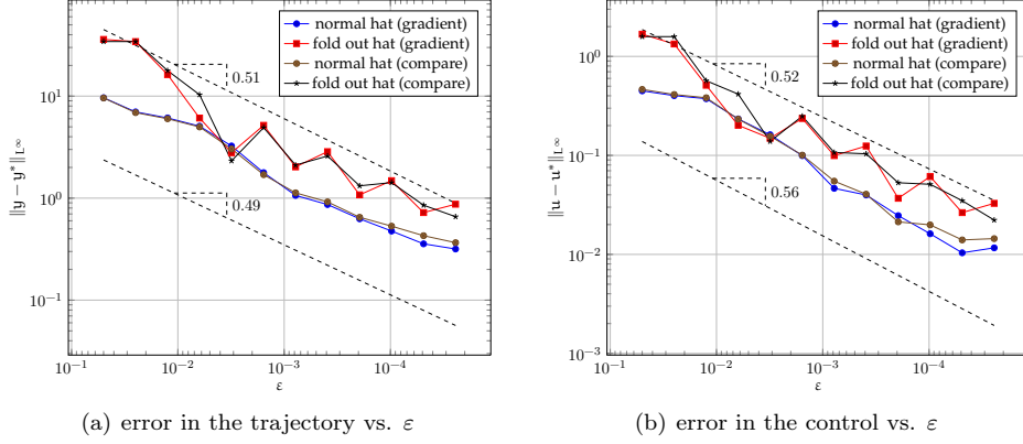
FIGURE 5. Harmonic oscillator (6.9) in 2D: Comparing the scheme on adaptive sparse grids using normal hat and fold out basis functions.
