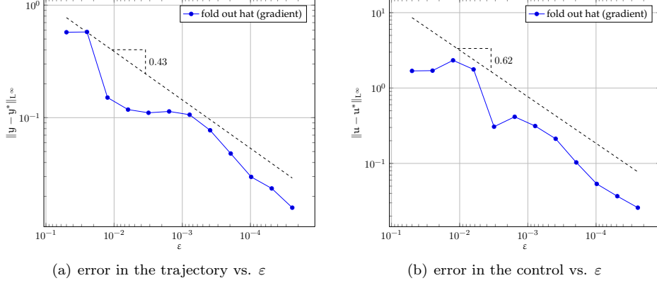
FIGURE 10. Wave equation (6.10) in 6D: The adaptive sparse grids scheme using fold out basis functions.
