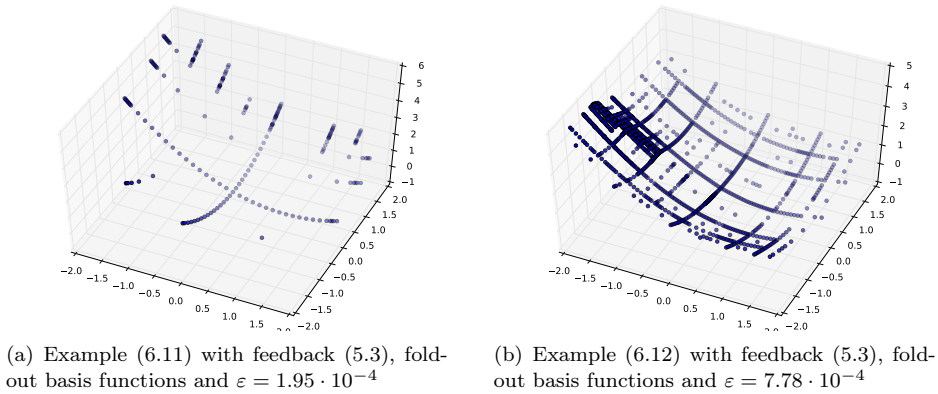
FIGURE 14. Bilinear equation (6.11) and (6.12) in 2D: Adaptive sparse grid.
