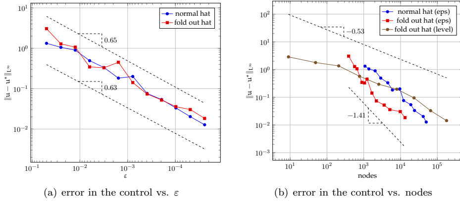
FIGURE 8. Wave equation (6.10) in 4D: Error in the control comparing the scheme based on sparse grids using normal hat and fold out basis functions, regular and adaptive sparse grids.
