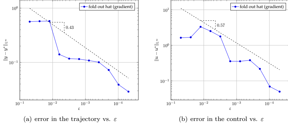
FIGURE 11. Wave equation (6.10) in 8D: The adaptive sparse grids scheme using fold out basis functions.
