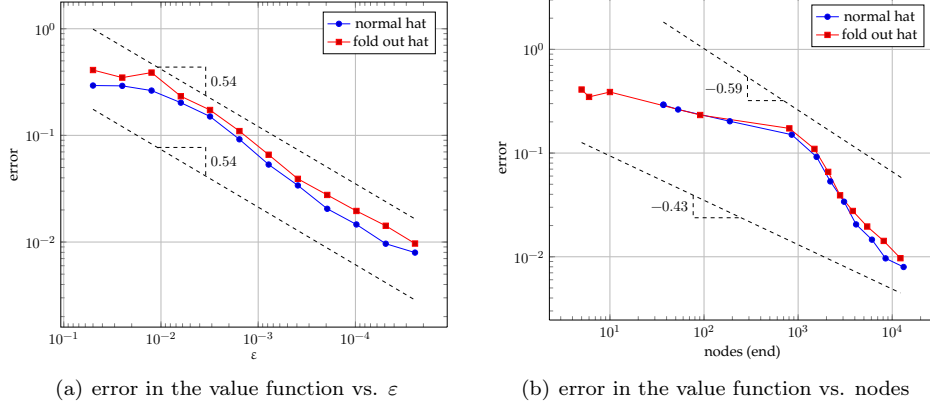
FIGURE 13. Bilinear equation (6.12) in 2D: Error in the value function comparing the scheme based on sparse grids using normal and fold out basis functions, adaptive sparse grid.
