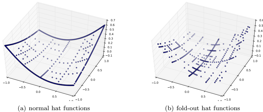
FIGURE 7. Harmonic oscillator (6.9) in 2D: Adaptive sparse grid for \varepsilon = 1.95 \cdot 10^{-4} .
