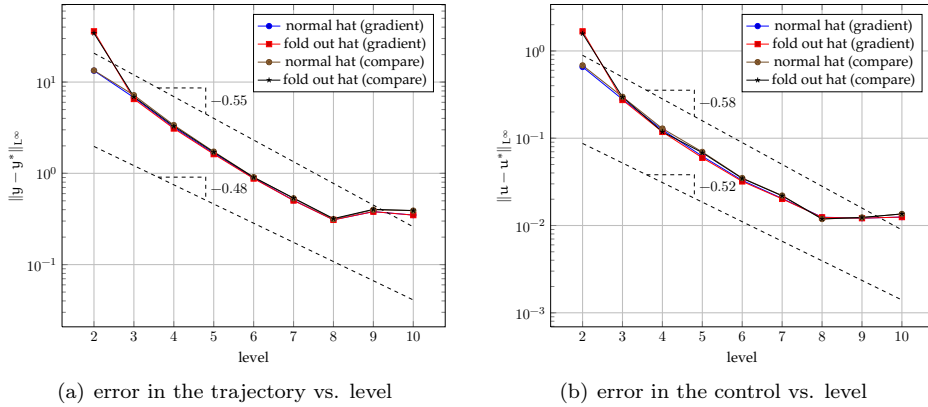
FIGURE 4. Harmonic oscillator (6.9) in 2D: Comparing the scheme on regular sparse grids using normal hat and fold out basis functions.
