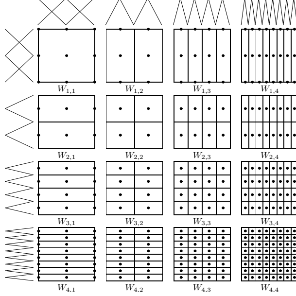
FIGURE 1. Supports of the basis functions \varphi_{L,j} of the hierarchical subspaces W_L of the space V_4 = V_{(4,4)} , where the functions of each W_L have disjoint support. The regular sparse grid V_4^s contains the upper left triangle of spaces.
