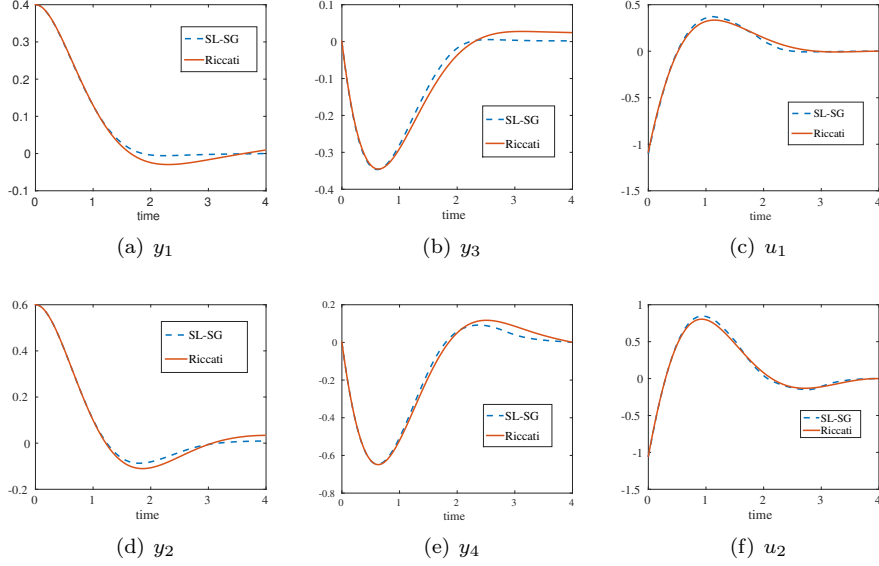
FIGURE 9. Wave equation (6.10) in 4D: Components of the optimal state y and corresponding optimal control u resulting from the SL-SG approach on a sparse grid with threshold \varepsilon = 2.44 \cdot 10^{-5} . As a reference solution the corresponding components of a solution generated by a Riccati approach are presented.
