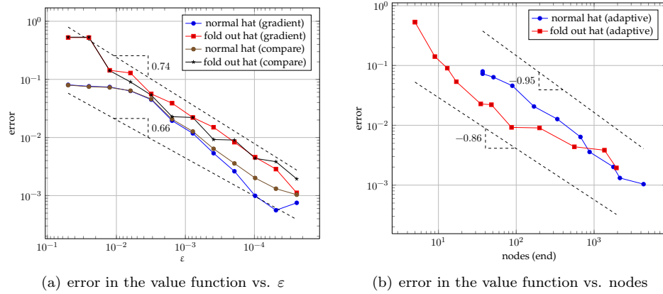
FIGURE 12. Bilinear equation (6.11): Error in the value function comparing the scheme based on sparse grids using normal and fold out basis functions, adaptive sparse grid (2D).
