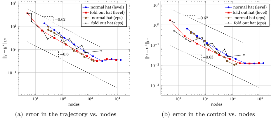
FIGURE 6. Harmonic oscillator (6.9) in 2D: Comparing the scheme using the gradient approach (5.2.2) on adaptive and regular sparse grids using normal hat and fold out basis functions.
