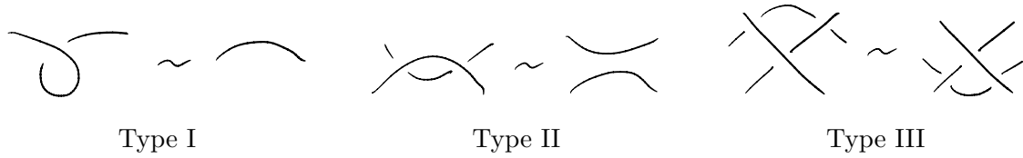
Figure 7.2.: Reidemeister Moves
