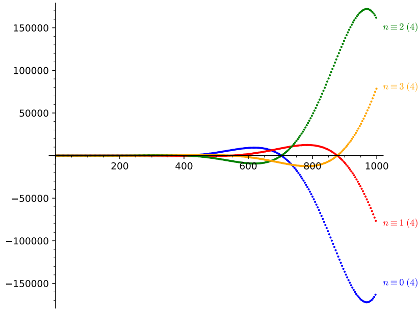
Figure 10.1.: V_1(n) for n \leq 1000
