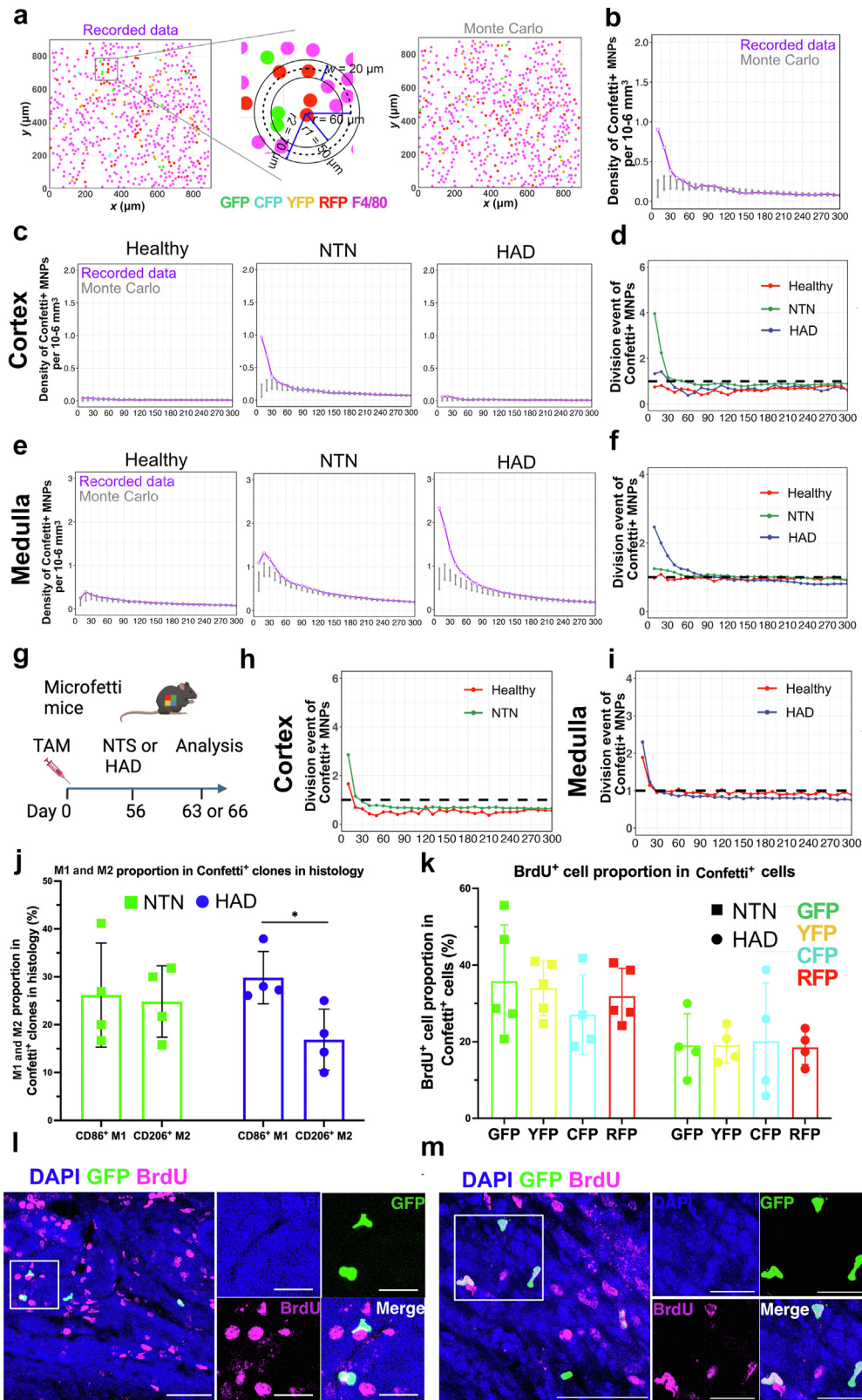
Figure 2 | Clonal intrarenal expansion of mononuclear phagocytes (MNP) in nephrotic nephritis (NTN) and high adenine diet (HAD). (a) Strategy for analysis of distribution of renal Confetti + MNPs. For each individual Confetti + MNP in a confocal stack (left), the density in concentric rings of 20 μm width (w) and radii (r) from 10 to 300 μm was determined, here illustrated for 60-μm radius as an example (middle). Monte Carlo (MC) simulation (right) of random distribution of renal Confetti + MNPs was performed 100 times to calculate the baseline density for MNPs that would result randomly. (b) Example of the MNP density (y axis) calculated by dividing corresponding same-color Confetti MNP counts by the ring volume of each ring size (x axis). The data density is shown in purple, and that of MC-simulated data is shown in (continued)
