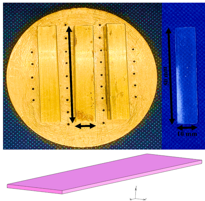
Fig. 1. A custom-made metal mold used for thermoforming of aligners sheets to produce test specimens in specific dimensions (Upper left), a test specimen in the form of rectangular strip (50 × 10 × 0.6 mm) (Upper right), a 3D model used for the 3D printing of strips made from TC-85 aligner material with the following dimensions: X = 50 mm, Y = 10 mm, Z = 0.6 mm (Lower).
