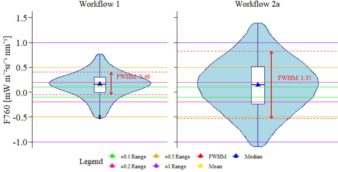
Figure 3.5: The violin plots represent the distribution of soil pixels retrieved F_{760} (mW m -2 sr -1 nm -1 ) using workflow 1 and 2a. The boxplot overlay shows the interquartile range and the median. The mean and median values are highlighted with yellow and blue points, respectively. Horizontal lines represent deviations from 0: ±0.1 (green), ±0.2 (pink), ±0.5 (orange), and ±1.0 (purple) mW m -2 sr -1 nm -1 . The red arrow indicates the Full Width at Half Maximum (FWHM).
