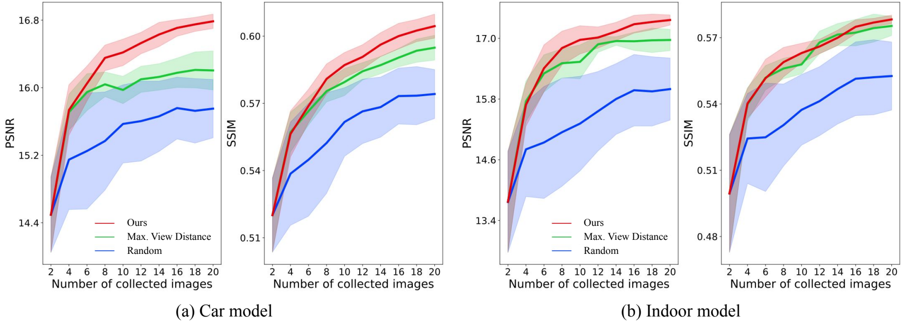
Figure 4.6: Comparison of NBV planners in a ShapeNet-based simulation environment. We conduct the experiments on (a) car and (b) indoor models, respectively. We precollect 100 test views for evaluation purposes. For each test viewpoint, we query a maximum of 5 closest reference images from currently collected images and use our image-based neural rendering network to render the test view. We report the average PSNR and SSIM with standard deviations over all test views and experiment runs. Our uncertainty-guided NBV planning outperforms non-adaptive heuristic baselines in finding more informative images, resulting in higher rendering quality given a limited measurement budget.
