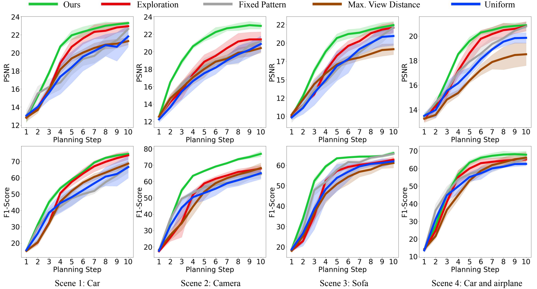
Figure 5.4: Comparison of reconstruction quality of objects of interest using different planning strategies in the four test scenes shown in Figure 5.3. We report the average PSNR and F1-score at each planning step. Solid lines show means over 5 trials and shaded regions indicate standard deviations. Our semantic-targeted approach exploits semantics in our implicit neural representation to achieve targeted view planning, leading to better and more stable reconstruction performance.
