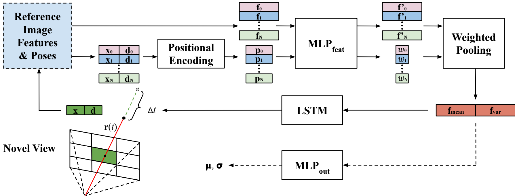
Figure 4.3: Our network architecture. Different colors indicate features from different reference images. Note that the encoder is not explicitly shown. We use a long short-term memory module to predict jumping distance \Delta t to the next sampling point, given the aggregated feature from all reference images acquired at the current sampling point. After a fixed number of iterations, the aggregated feature at the final point is interpreted to color and uncertainty information. Arrows with dashed lines show the forward pass happening only in the last iteration.
