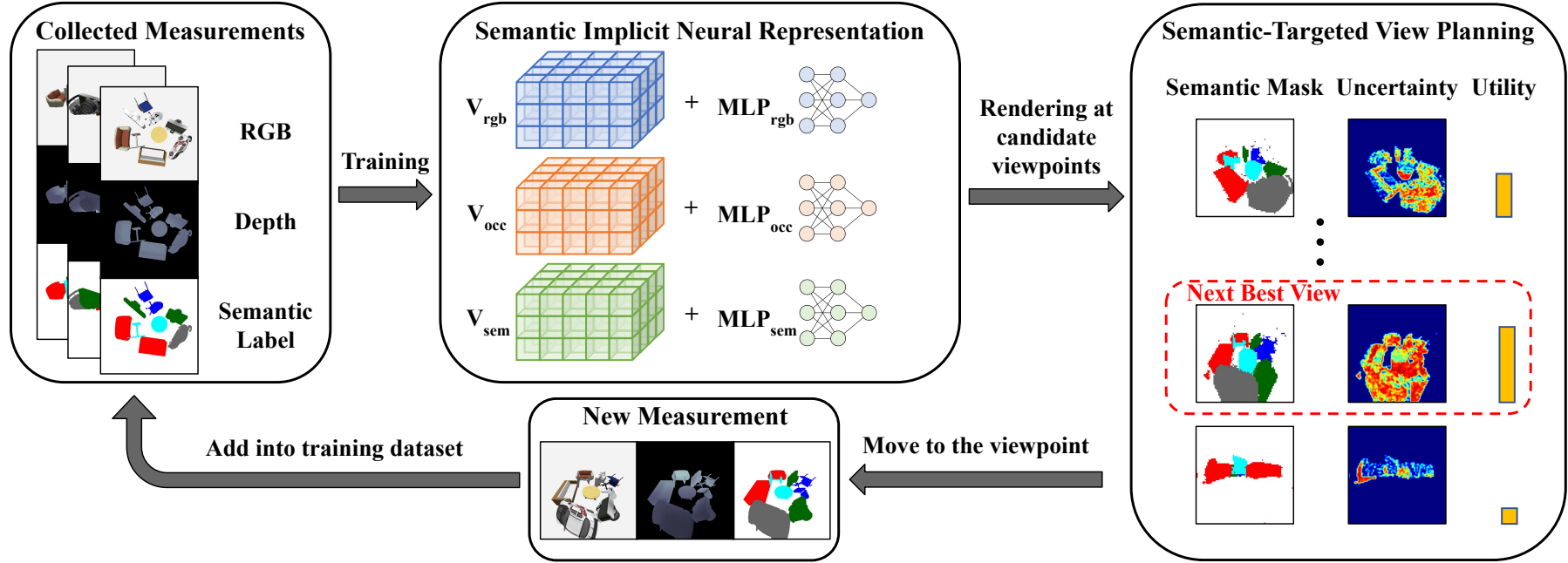
Figure 5.2: Overview of our proposed approach, STAIR. We incrementally train our semantic implicit neural representation using posed RGB-D measurements and their 2D semantic labels. After training, we render semantics and uncertainty at sampled candidate viewpoints. For planning, our utility function considers both overall view uncertainty and the uncertainty from objects of interest. We select the candidate viewpoint with the highest utility value as our next measurement location. We iterate between map representation training and view planning until a maximum allowable number of measurements is reached.
