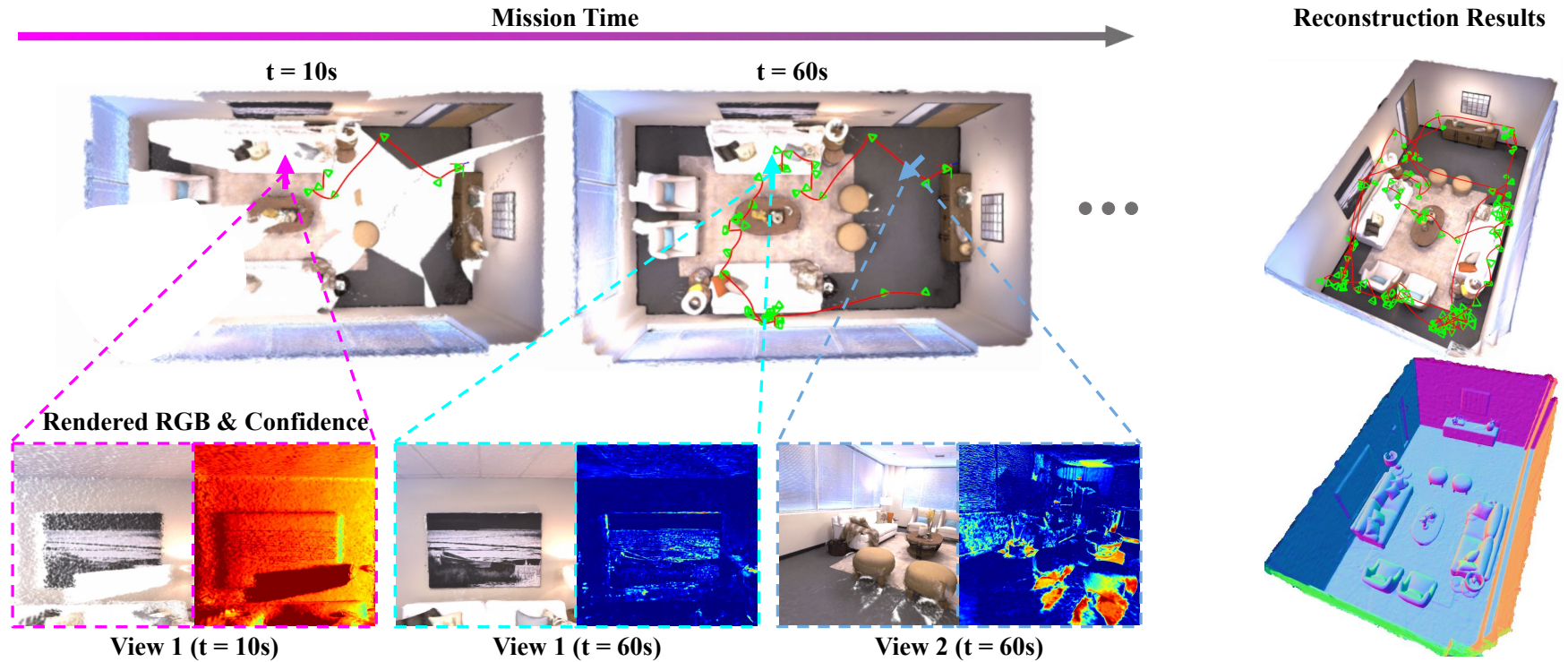
Figure 6.1: Our approach actively reconstructs an unknown scene. We illustrate the reconstruction progress over mission time, displaying planned camera viewpoints (green pyramids) and paths (red lines). We present examples of RGB and confidence images (redder color indicates lower confidence) rendered at the same viewpoint at different mission times (magenta and cyan arrows) and at two distinct viewpoints at the same mission time (cyan and blue arrows). By integrating confidence modeling into the Gaussian splatting pipeline, our approach enables targeted view planning to build a high-fidelity GS map. The complete camera path and final reconstruction results, including RGB rendering and surface mesh, are visualized on the right.
