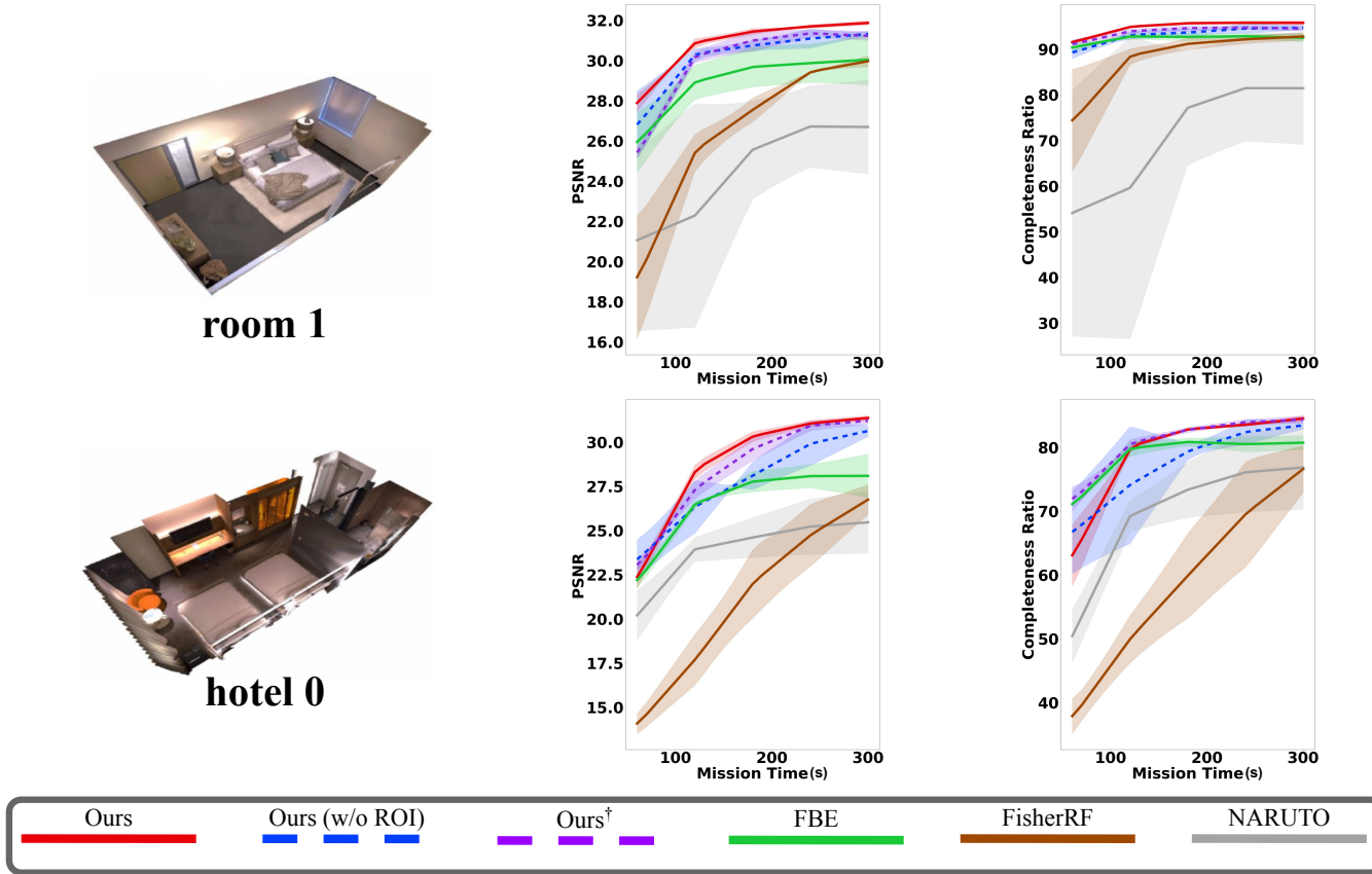
Figure 6.4: We report the reconstruction performance evaluated in rendering and mesh quality over online mission time. Our ActiveGS outperforms baselines in all test scenes. Our view planner considers unexplored regions for exploration, while exploiting low-confidence Gaussian primitives for further inspection. Compared to GS-based approaches, our approach proposes explicit confidence modeling of Gaussian primitives, enabling targeted candidate viewpoint generation and fast viewpoint evaluation. Our approaches demonstrate a large performance gain over the state-of-the-art NeRF-based approach, NARUTO , motivating the use of GS in active scene reconstruction.
