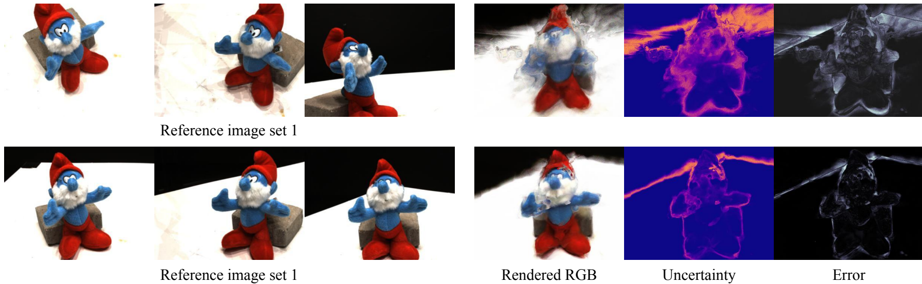
Figure 4.4: Examples of our input-dependent uncertainty estimation in image-based neural rendering. For rendering the same novel view, we select two sets of reference images. The comparison clearly shows how rendering quality depends on the scene information provided by reference images. Reference images with low information value lead to blurry rendering and correspondingly high uncertainty prediction (yellow) from our network. The error map shows the mean squared error between ground truth and rendered RGB (whiter areas indicate higher errors). Our uncertainty prediction is strongly correlated with this error, thus serving as a good proxy for view planning.
