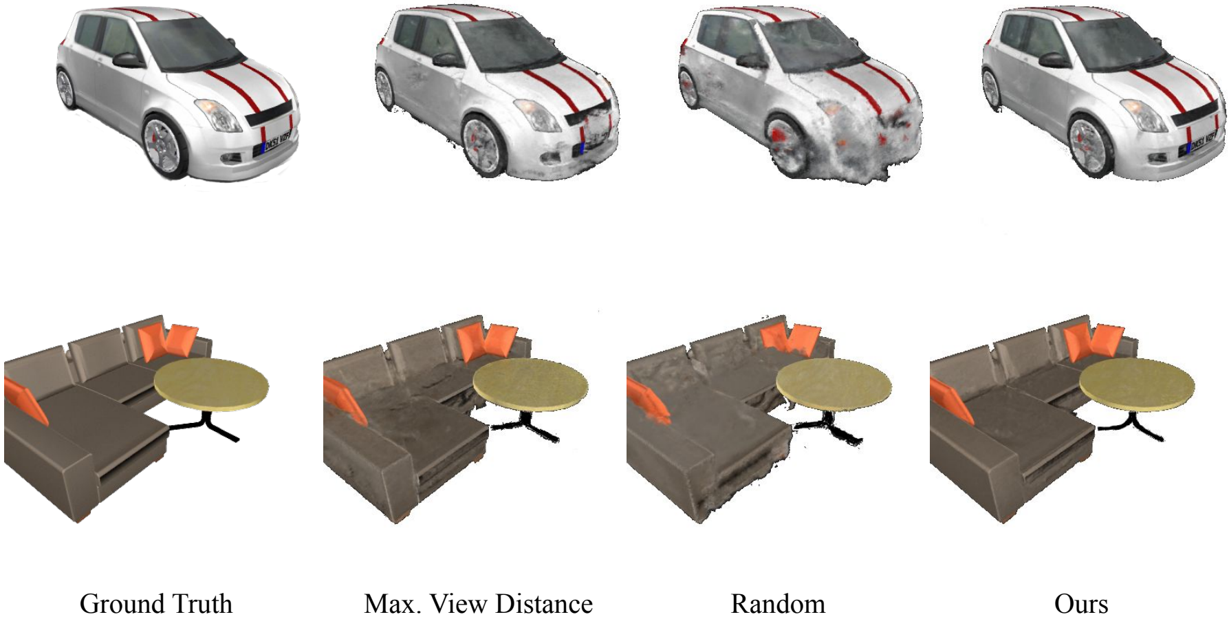
Figure 4.7: Qualitative rendering results of offline trained NeRFs using image collections from three different NBV planners. We select a challenging view from each scene to show the rendering quality differences. Our uncertainty-guided planner adapts the acquisition of new measurements according to the scene structure, in contrast to the heuristic strategies. For example, our approach takes more images of the car bonnet, which has more structural details compared to the car sides and is thus difficult to model using sparse reference images.
