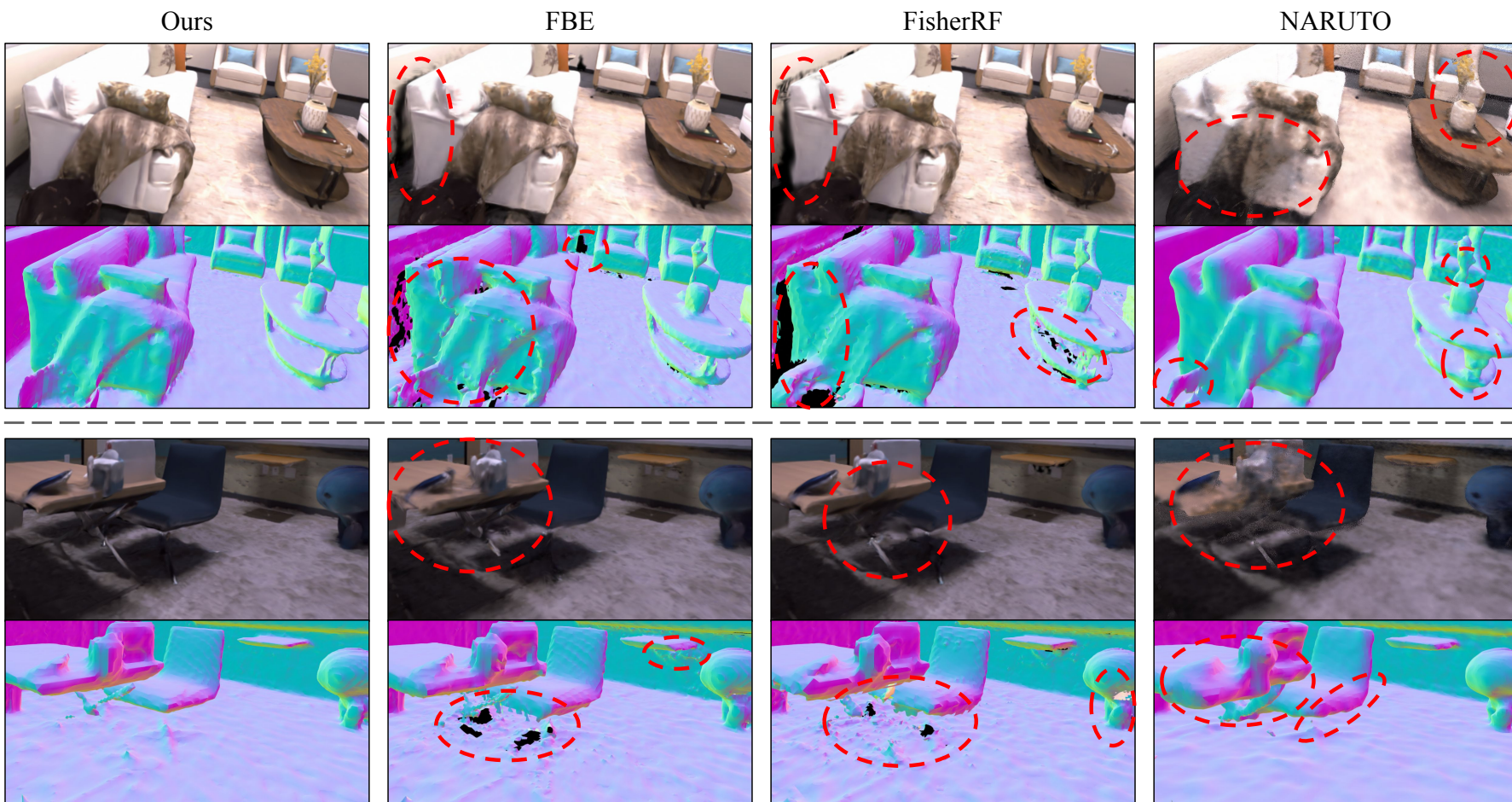
Figure 6.5: Visual comparison of reconstruction results using different approaches. We show RGB rendering and surface meshes for two scenes, with red circles highlighting areas of low-quality reconstruction from baseline approaches. Our ActiveGS considers both unexplored regions in voxel map and confidence value of GS map to enable targeted view planning, achieving complete and high-fidelity scene reconstruction.
