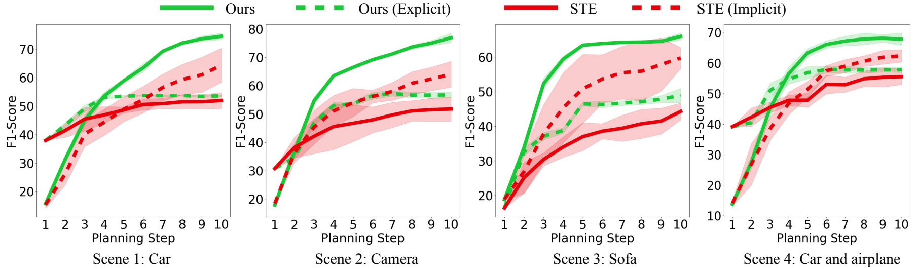
Figure 5.6: Comparison of our approach against the semantic-targeted active explicit reconstruction system STE [208]. Dashed lines denote variants cross-validating the measurements collected by one active reconstruction system with the mapping method of the other. The same color indicates mapping using the same measurements. The results confirm that our STAIR pipeline achieves superior performance compared to the explicit baseline. The performance gain originates from the implicit neural representation used in our approach and our utility function for finding more informative measurements.
