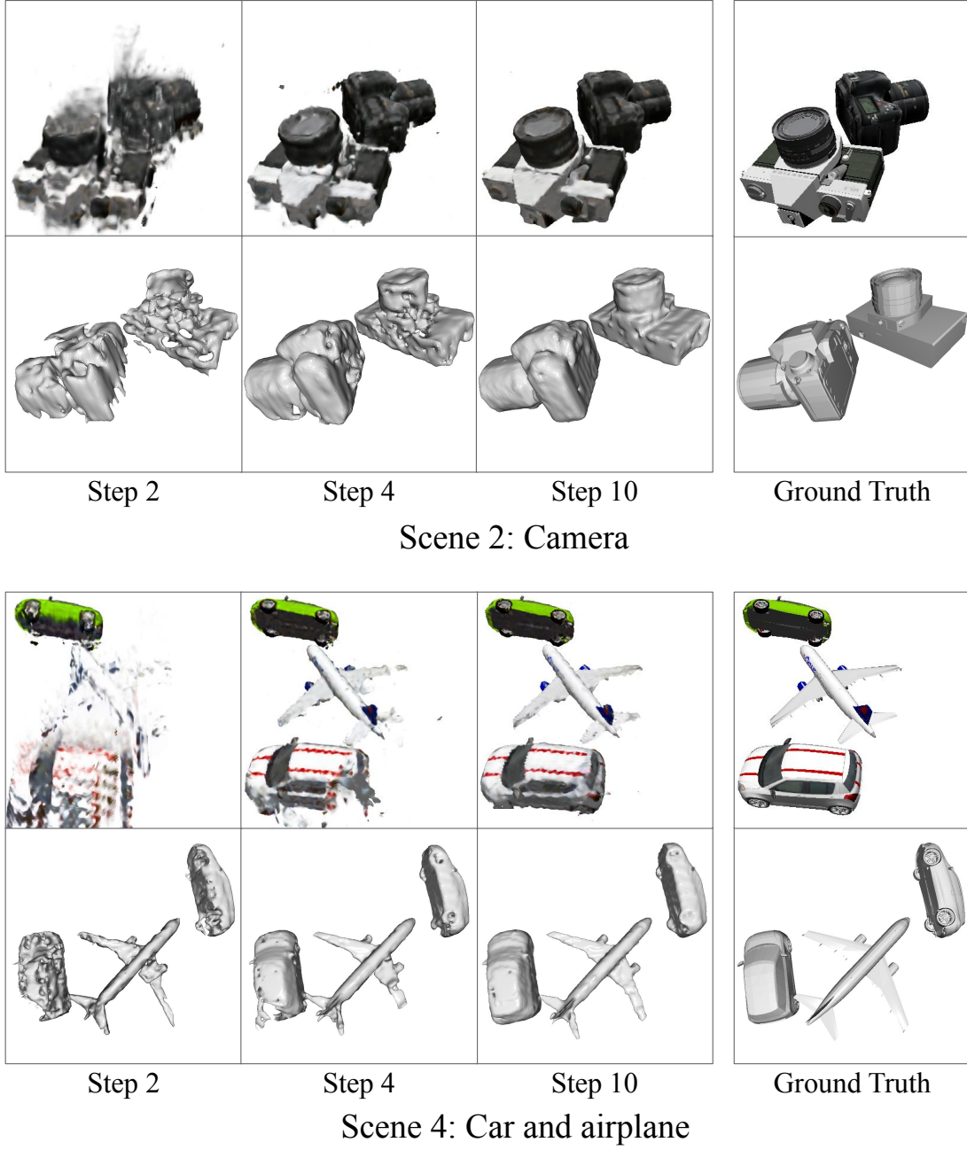
Figure 5.5: Qualitative results of our approach showing how novel view rendering (top) and meshes (bottom) improve along planning steps during a mission. Our approach collects informative measurements about objects of interest in a targeted way to achieve high-quality reconstruction.
