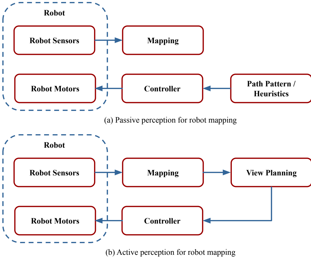
Figure 1.3: A comparison between the general frameworks of passive and active perception for robot mapping. (a) In passive perception, the robot follows a predefined path or non-adaptive heuristic to collect measurements for mapping, which may result in redundant or incomplete measurements of the environment, leading to inefficient or low-quality mapping. (b) In contrast, active perception enables the robot to actively select informative viewpoints based on the current map state, directly optimizing specific mapping objectives, such as full coverage or high reconstruction accuracy. This closed-loop setup enhances the robot autonomy and leads to more efficient and accurate mapping in unknown environments.
