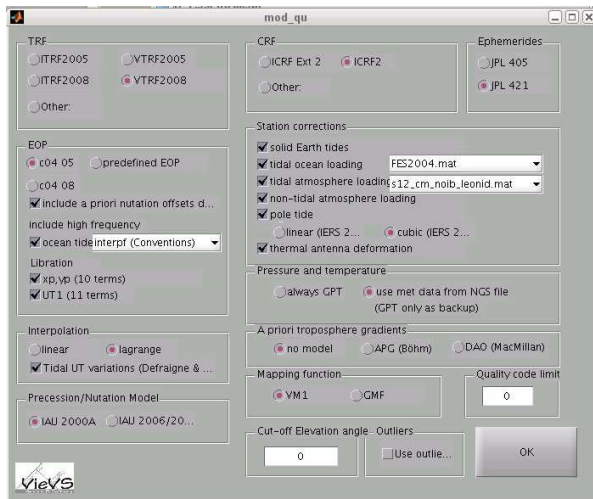
Fig. 2 Part of the VieVS Graphical User Interface. This part is for selecting the models to be used in VIE_INIT and VIE_MOD.
