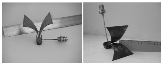
Fig. 1 Photos of the manufactured TEM horn feeds.
