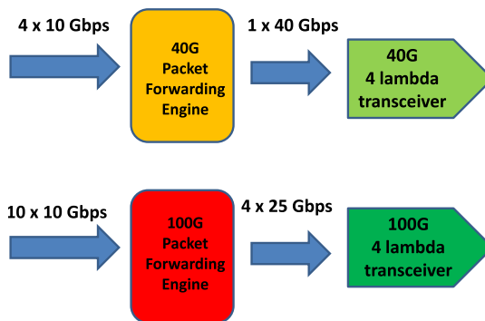
Fig. 4 The Network Board FILA40G
