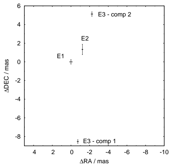
Fig. 3 Relative change in position for AC211. The bipolar structure observed in epoch 3 is still under investigation.
