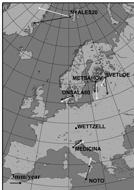
Fig. 6 Horizontal velocities derived from IVS-T2 VLBI campaign (white arrows) and GPS data (black arrows).
