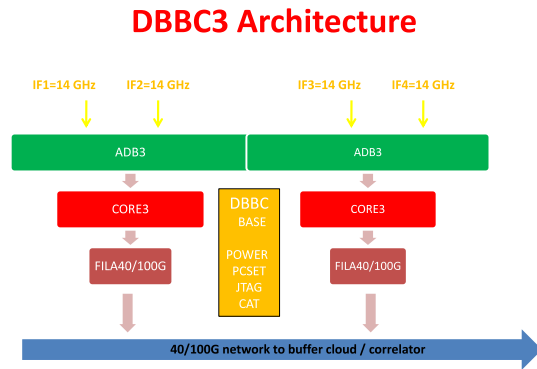
Fig. 1 DBBC3 Architecture
