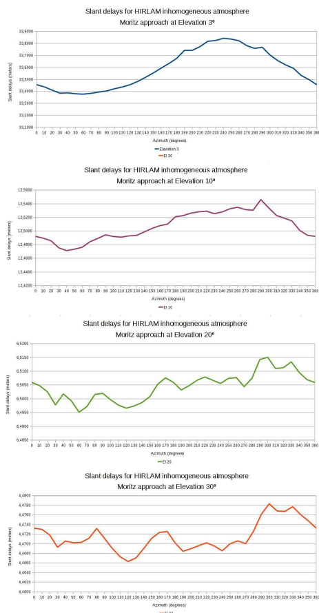
Fig. 5 Calculated slant delays for elevation angles 3°, 10°, 20° and 30° in an inhomogeneous atmosphere using the Conformal Theory of Refraction through HIRLAM for Effelsberg station (25 th March 2005 at 12:00 - start time for EURO75).
