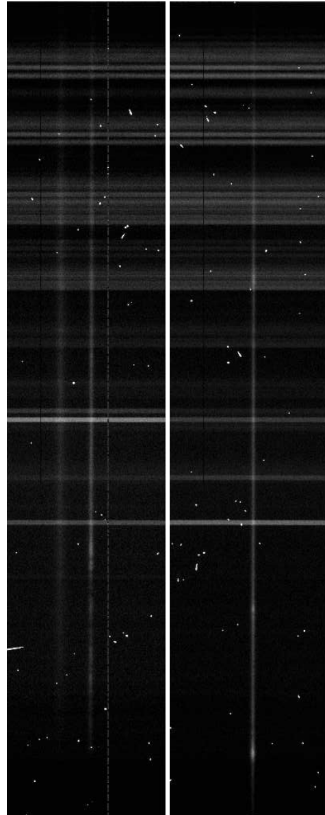
Fig. 1 Unprocessed spectra of IVS B1505–304 (left) and B2354–251 (right). The wavelength range is from 3685Å at the bottom to 9315 Å at the top. Vertical lines across the centre of the images represent continuum spectrum of the objects, and bright spots indicate positions of emission lines.
