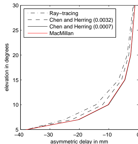
Fig. 1 Asymmetric delays towards east at station Wetzell on 1 January 2008. The gradient mapping functions were scaled to agree with the ray-traced delays at 5 degrees elevation. A coefficient C of about 0.0060 would agree best with the ray-traced delays in the range of elevations shown in the figure.
