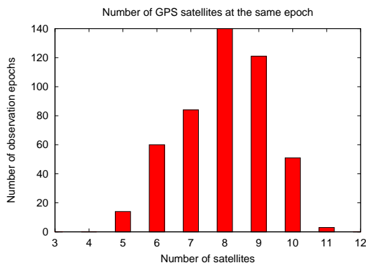
Fig. 3 Number of simultaneously observed GPS satellites above 15 degree cutoff angle in elevation
