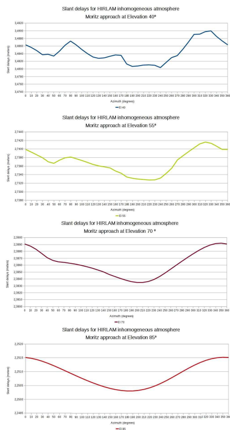
Fig. 6 Calculated slant delays for elevation angles 40°, 55°, 70° and 85° in an inhomogeneous atmosphere using the Conformal Theory of Refraction through HIRLAM for Effelsberg station (25 th March 2005 at 12:00 - start time for EURO75).
