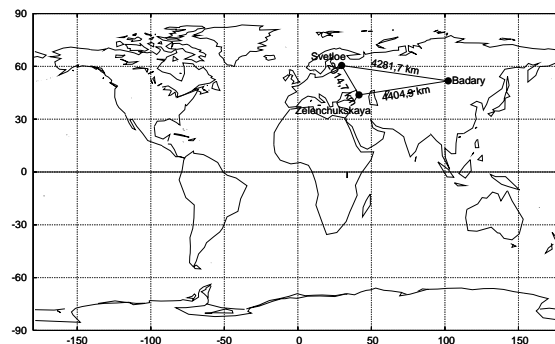
Fig. 1 "Quasar" network
