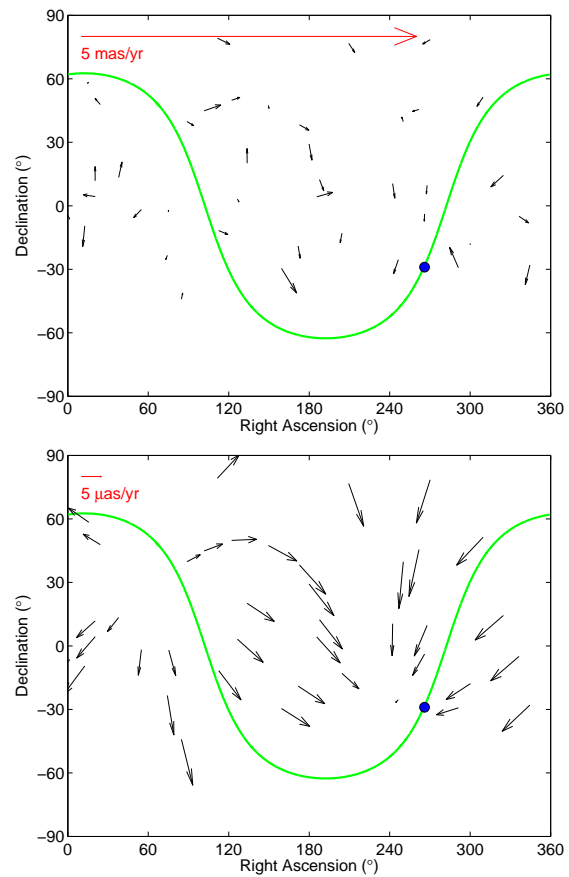
Fig. 2 Velocities and dipole pattern obtained from the 40 most observed sources. Solid line with dot shows the Galactic plane and the Galactic centre.
