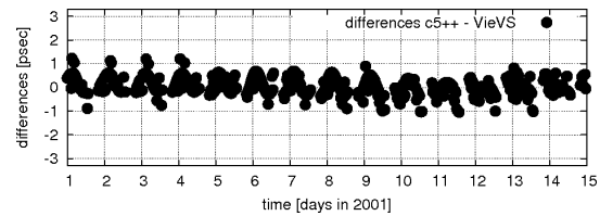
Fig. 4 Differences of total theoretical delay for the baseline Westford-Wettzell between c5++ and VieVS as obtained within DeDeCC (after Hobiger et al., 2010).
