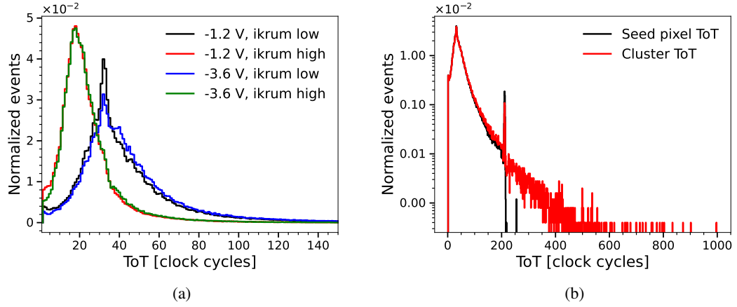
Figure 7.13: (a) Seed pixel ToT distribution for two different feedback currents and sensor bias voltages. The threshold is approximately 300 electrons. (b) Seed pixel and cluster ToT distributions for the low ikrum setting and sensor bias voltage of -1.2 V.
