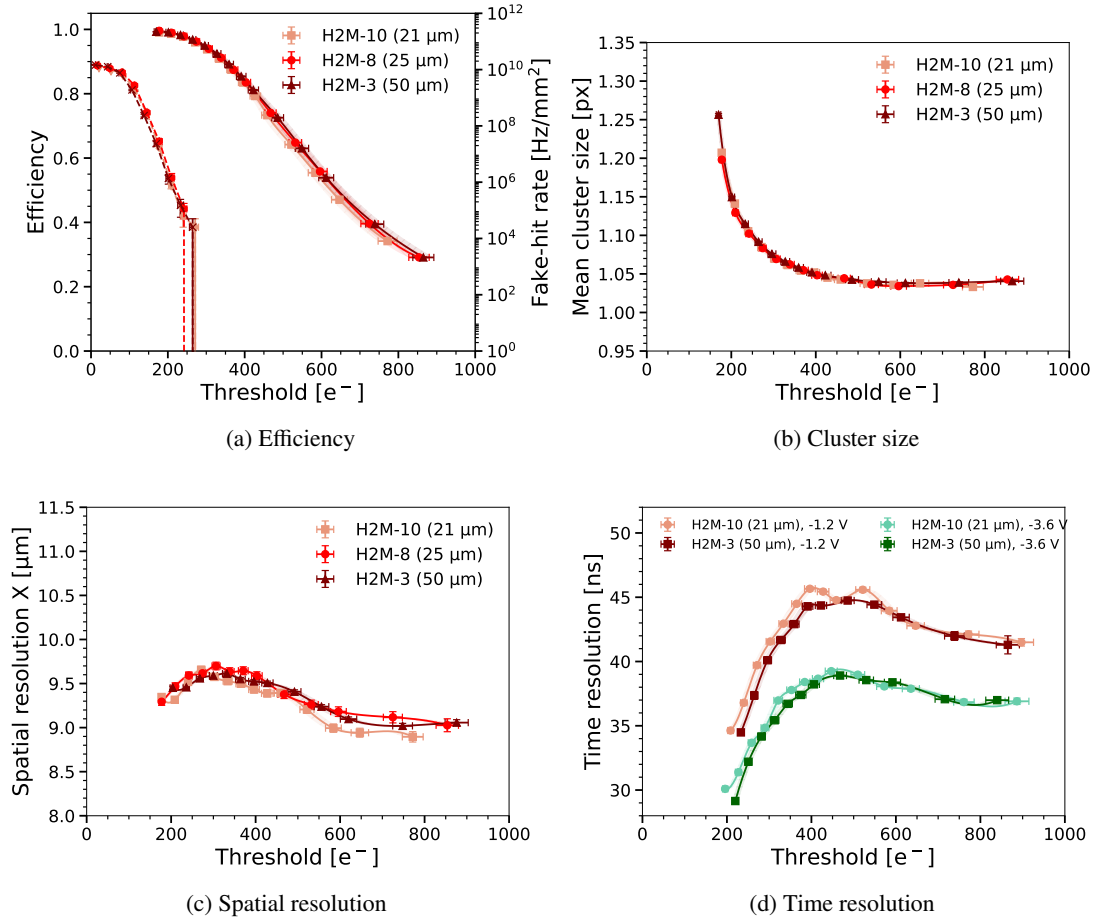
Figure 7.24: Efficiency and fake-hit rate (a), cluster size (b), spatial (c) and time (d) resolution as a function of the threshold for samples with different total chip thicknesses. In (a), (b), and (c), the data is recorded in triggered mode and the sensor is biased at -1.2 V. In (d), the data is measured in triggered mode. The low ikrum setting is used for all plots. The uncertainty is dominated by the threshold calibration factor, which is represented by a band.
