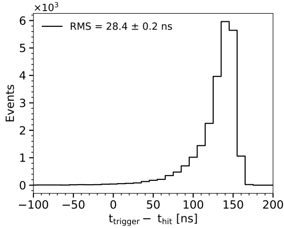
Figure 7.19: Time residual distribution. The sensor is biased at -3.6 V, the threshold is 224 electrons, and a low ikrum setting is used.
