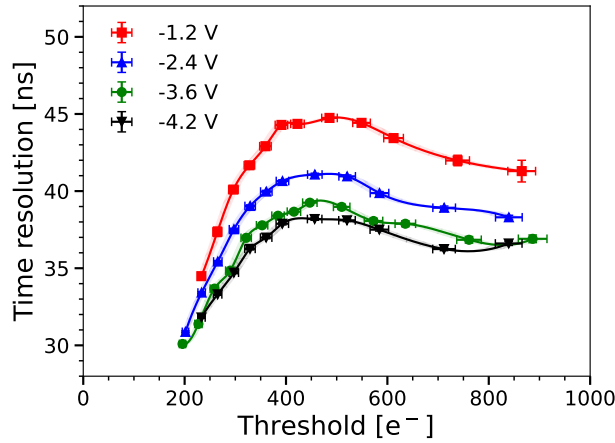
Figure 7.21: Time resolution as a function of the threshold for different sensor bias voltages. A low i_{krum} is used. The uncertainty is dominated by the threshold calibration factor, which is represented by a band.
