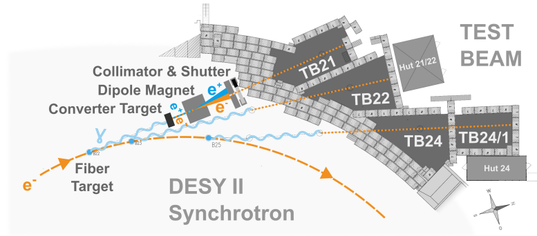
Figure 6.1: Schematic layout of the beam production and extraction at the DESY II test beam facility. Taken from [137].
