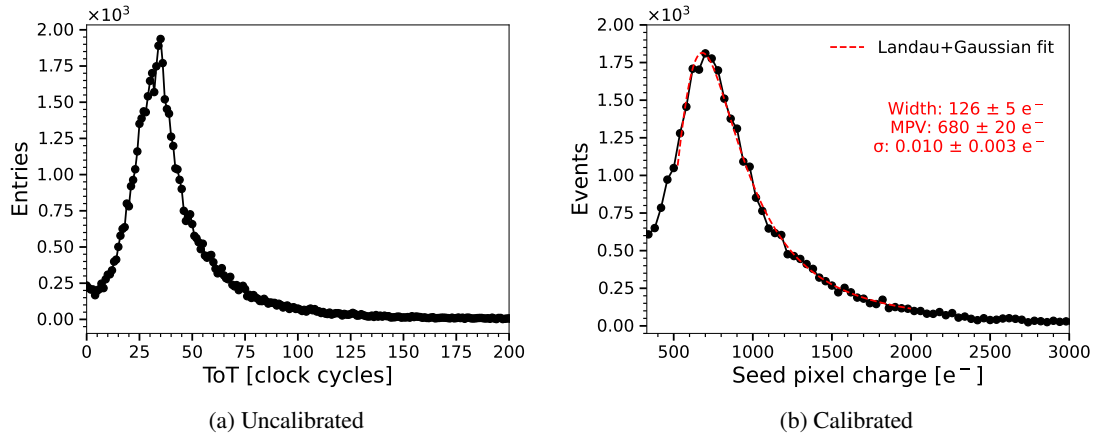
Figure 7.14: Seed-pixel charge distribution before (a) and after (b) calibration. The sensor is biased at -1.2 V, the threshold is approximately 300 electrons, and the low ikrum setting is used. For the calibrated distribution, a Landau-Gaussian convolution is used for fitting. The fit parameters of the width and MPV of the Landau distribution, and the standard deviation of the Gaussian component \sigma , are displayed.
