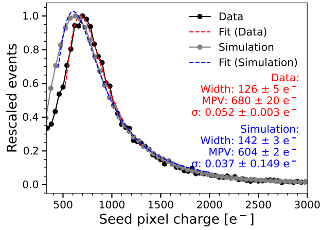
Figure 8.6: Comparison of seed-pixel charge distributions between data and simulations. The threshold is 300 electrons, and the sensor bias -1.2 V. A low ikrum is used in measurements. The measurement distribution is presented in Figure 7.14(b), and the simulation distribution in Figure 4.8.
