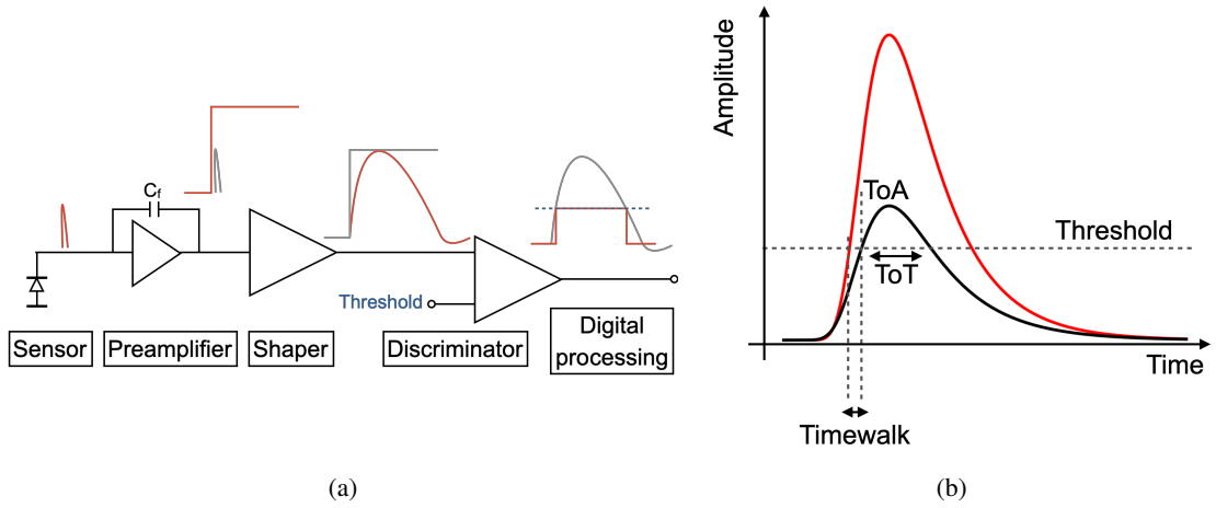
Figure 2.3: Typical readout scheme for a silicon pixel detector in HEP. Adapted from [8]. (b) Sketch of two signals with different amplitudes and timewalk. For the smallest signal, the ToT and ToA are indicated.
