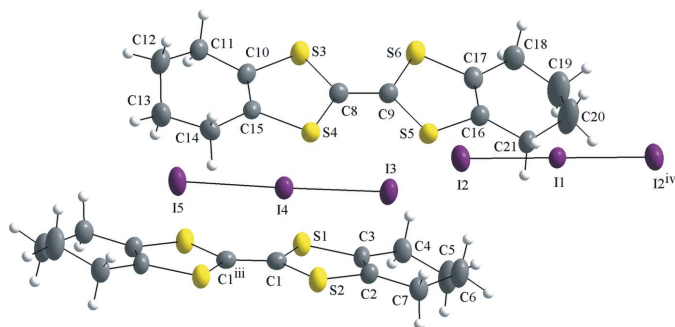
Figure 1 The molecular structure of the title compound, \delta -(OMTTF)I 3 , showing the atom labelling and displacement ellipsoids drawn at the 40% probability level. Symmetry codes: (iii) -x + 1, -y + 1, -z ; (iv) -x + 2, -y, -z + 1 .
