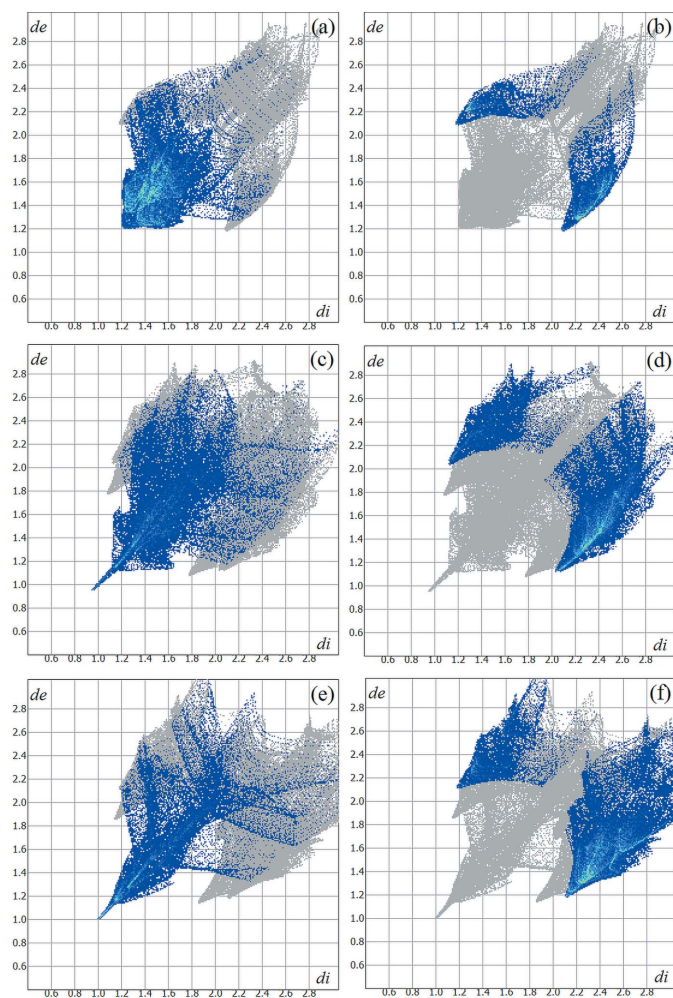
Figure 7 Two-dimensional Hirshfeld surface fingerprint plots for the \alpha , \beta and \gamma (OMTTF ^{+\bullet} )(I _3^- ) crystalline modifications. The H \cdots H and H \cdots I intermolecular contacts are drawn as cyan dots. The contributions of these interactions for the crystal packing of the \alpha form amount to (a) 43.30% and (b) 17.40%, respectively. For the \beta form the values amount to (c) 29.20% and (d) 33.90% and, finally, for the \gamma form the values are (e) 23.00% and (f) 39.70%.
