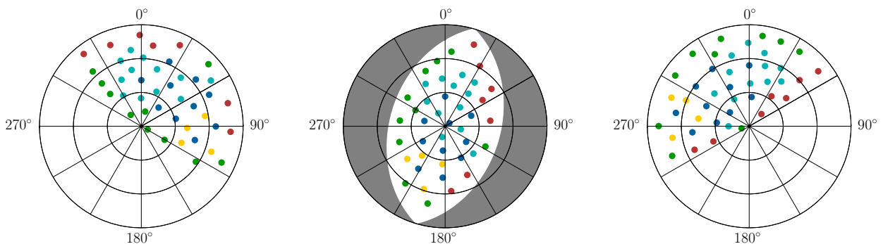
Figure 3.6: Skyplot of Wettzell (left), the baselines mid-point (center) and Tsukuba (right) for the uniform sky scheduled test session with clustered observations.
