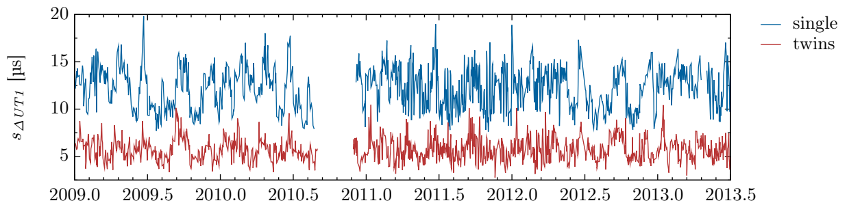
Figure 6.6: Comparison of \Delta UT1 repeatabilities with single and twin telescopes for INT1 sessions.
