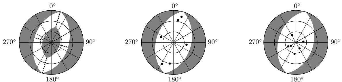
Figure 4.2: Locations of initial sources depicted at the skyplot of the baseline's mid point. Left: schematic geometric criteria. Middle: example for geometric criteria. Right: example for predicted precision of the observations.
