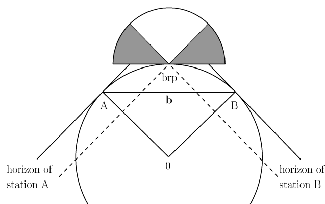
Figure 3.4: Geometry of baseline reference system and horizon mask (according to NOTHNAGEL and CAMPBELL 1991).
