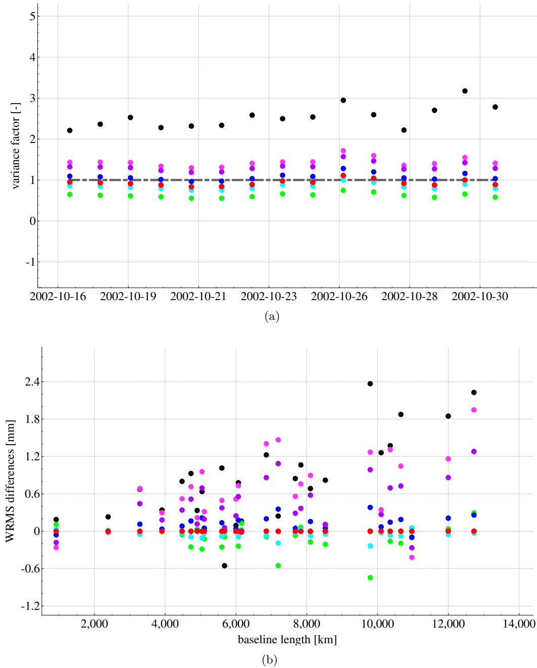
Figure 5.5: The influence of different turbulence parametrizations on the \chi^2 values and the VLBI target parameters in terms of the baseline length repeatabilities, plotted as difference with respect to the turbulence-based reference solution (setup 1; red). The black dots (setup 0) denote a solution without using a turbulence model. The solution with a modified structure constant (setup 2) is given by green dots, and a change of the effective tropospheric height is visualized by light (setup 3) and dark blue (setup 4) dots. A modification of the anisotropic scaling factors is represented by purple (setup 5) and magenta (setup 6) dots. Finally, a reduction in the wind velocity is visualized by orange dots (almost fully covered by the red dots).
