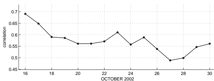
Figure 6.9: Level of correlations between the two contributions (IGG and BKG) during the two-week CONT02 campaign.
