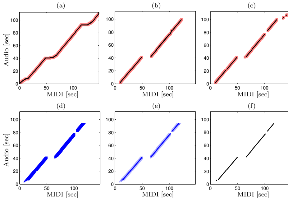
Figure 5.1. Steps in the proposed method continuing the example shown in Figure 4.1. (a)-(c) Alignment (black) and corresponding augmented binary matrix (red and white) for the optimal global path (DTW), family of paths (Smith-Waterman) and the optimal match (partial matching). (d) Intersection matrix derived from (a)-(c). (e) Weighted intersection matrix. (f) Consistency alignment \mathcal{C} .
