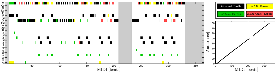
Figure 5.7. Cross-version chord evaluation for the song Getting Better . Left: Overlay of two MIDI-based chord labeling results ( Melisma and RLM ) and manually generated audio-based chord labels. Right: Consistency alignment (horizontal axis specifies MIDI time in beats and vertical axis specifies audio time in seconds).
