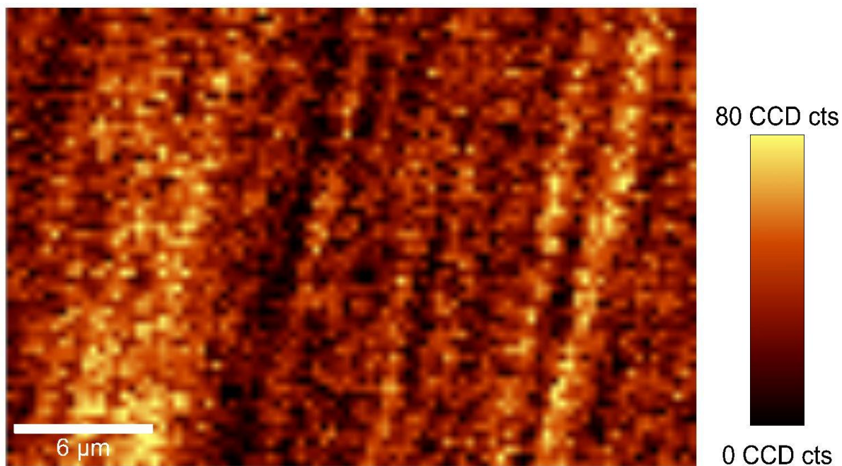
Figure 3 False colour images of the inner layer (layer thickness: 8 μm) containing 15 % poly(TBAMS) of the multilayer foil visualize the intensity of the vibration at 1607 cm -1 (C=C) of TBAMS in the scanned area
