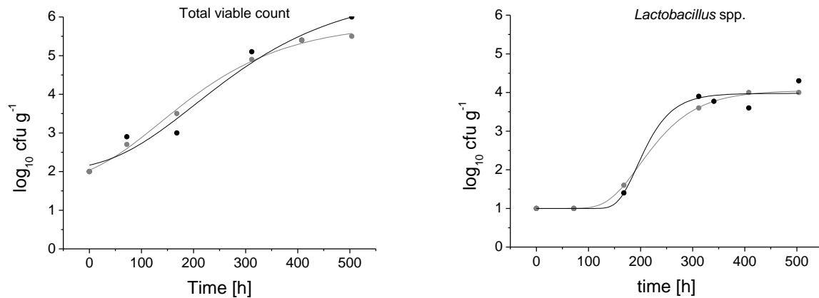
Figure 6 Growth of total viable count and Lactobacillus spp. on veal cutlets stored in reference foil and sample foil containing 10 % of poly(TBAMS) at a constant temperature of 2 °C. Bacterial counts (n = 4): (●) Reference foil and (●) Sample foil
